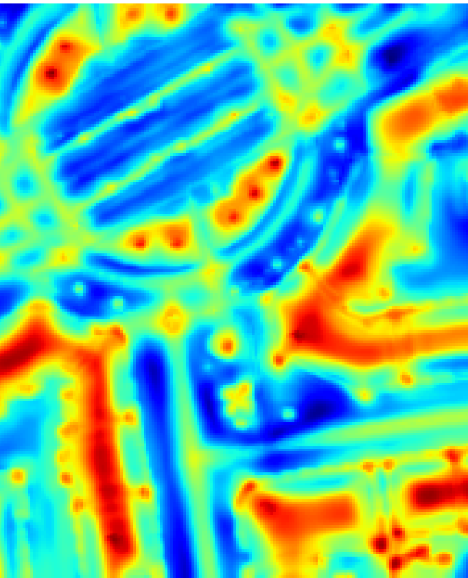
map norm
