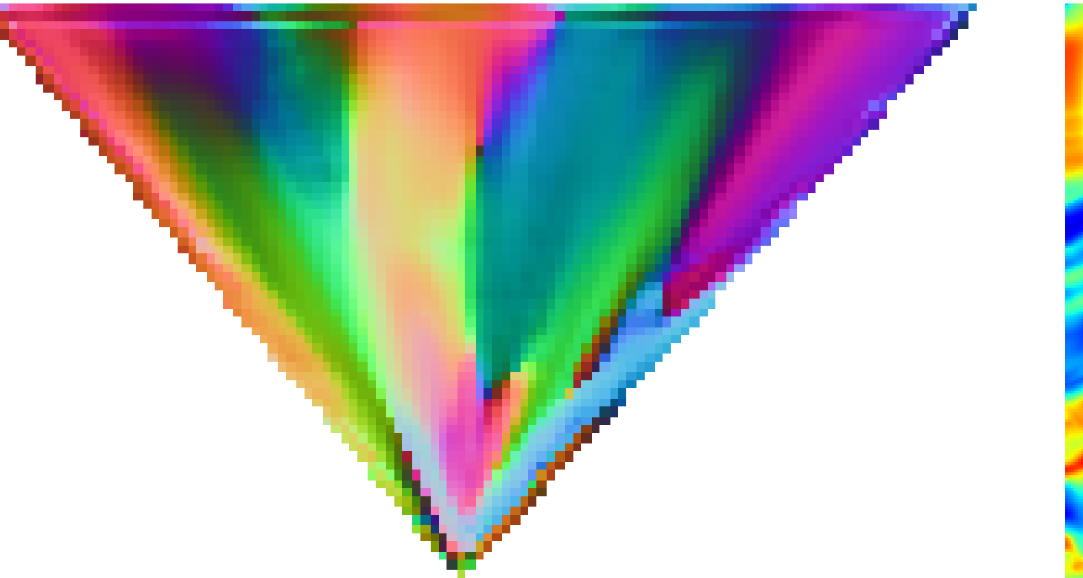
BEV features
