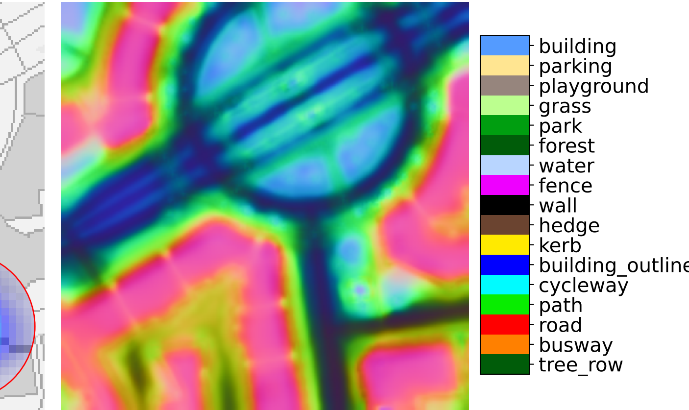
neural map
