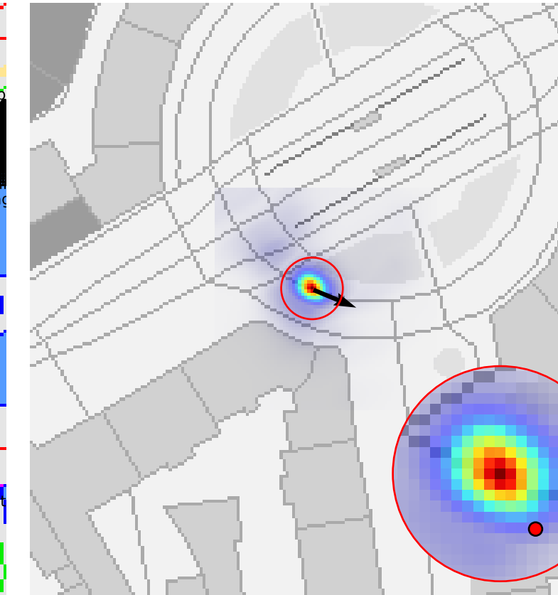
likelihood
