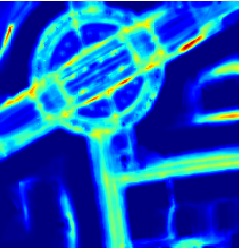
map prior
