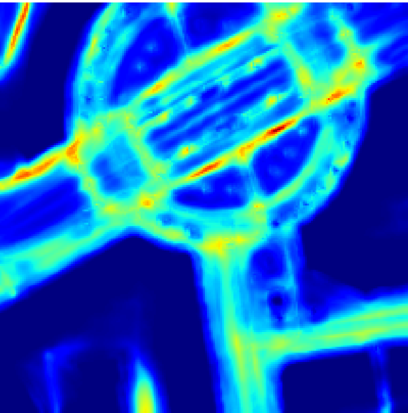
map prior
