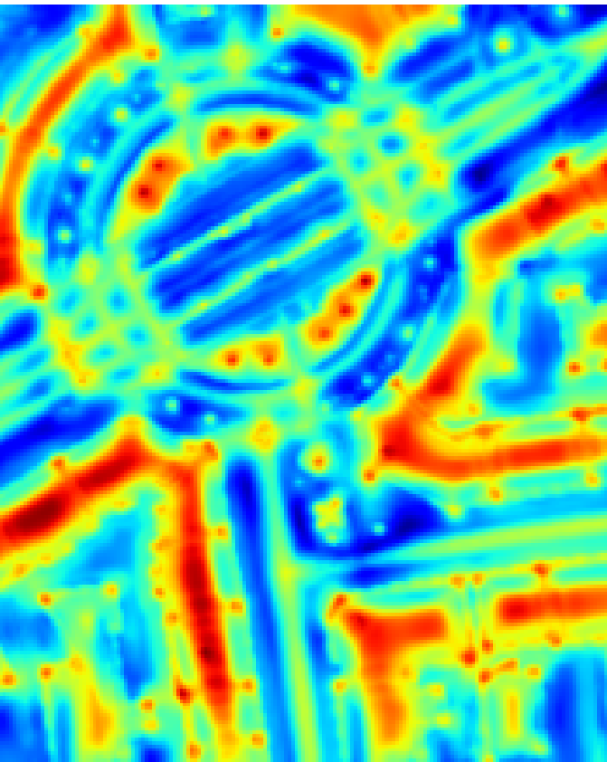
map norm
