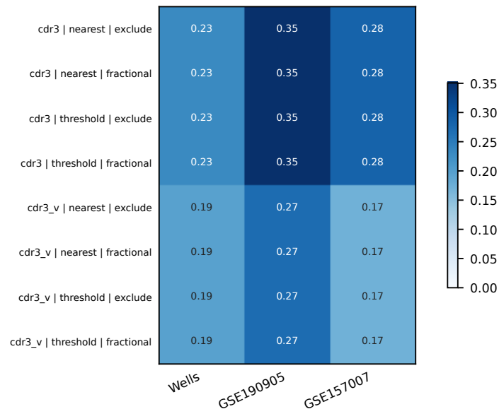
D Prespecified null sensitivity
