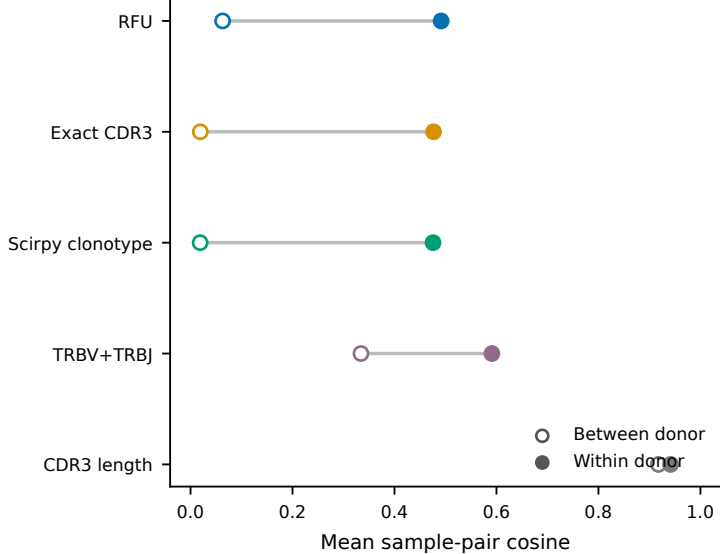
A Repeated samples retain donor structure
