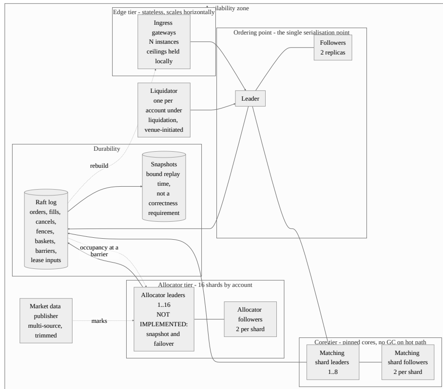
Figure 4: Deployment view. The target deployment; no part of it has been implemented or measured.
