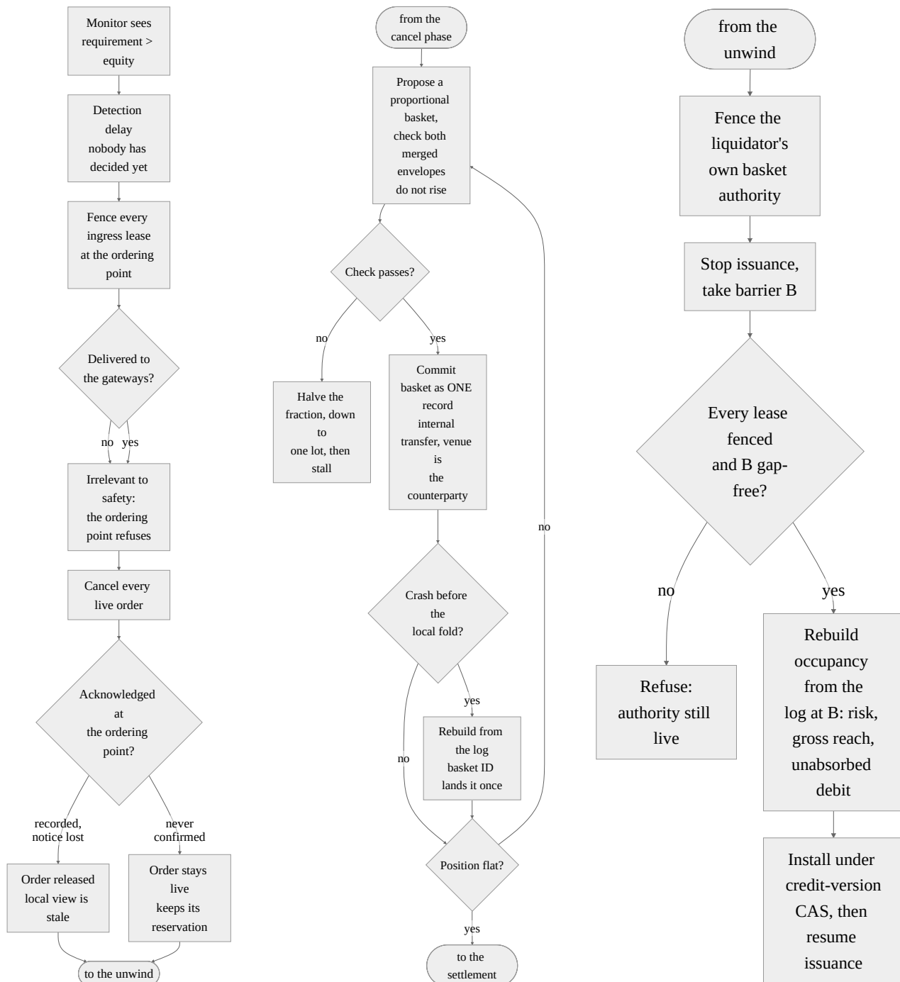
Figure 5: Liquidation and settlement. Stop, unwind, settle. The two exits from the cancel check are the two different facts of §5.4.
