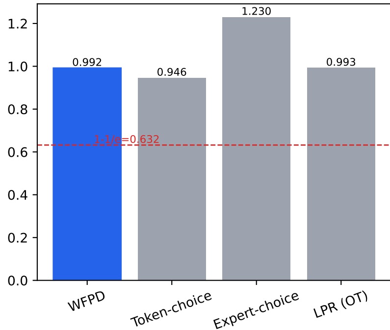
Retained score (ALG / OPT)
