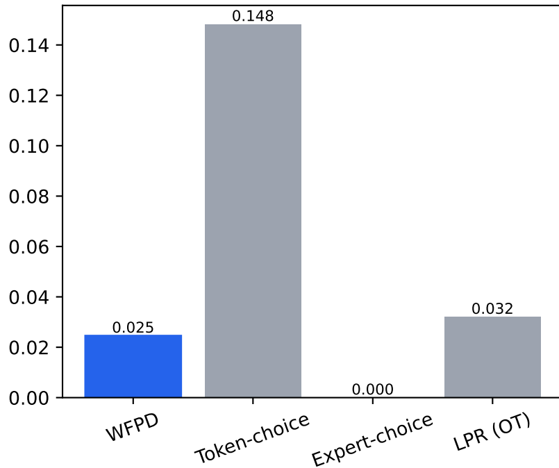
Load Gini (lower = better)
