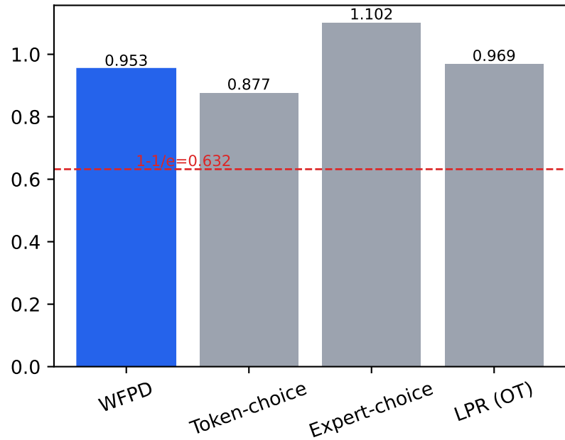
Retained score (ALG / OPT)
