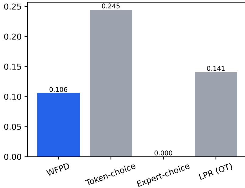
Load Gini (lower = better)
