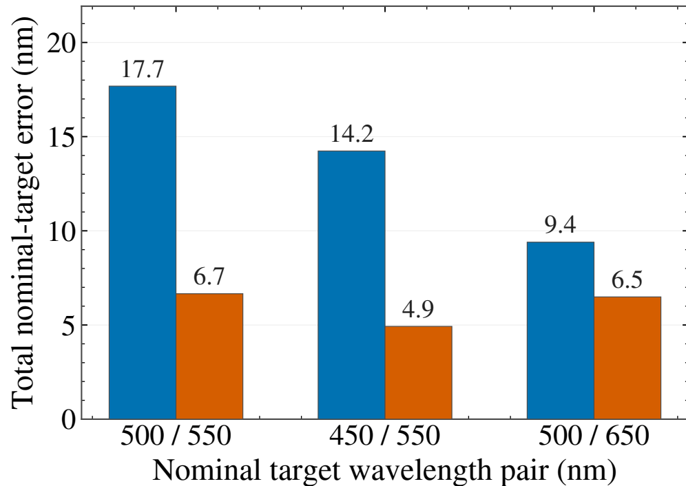
Double-notch filter
