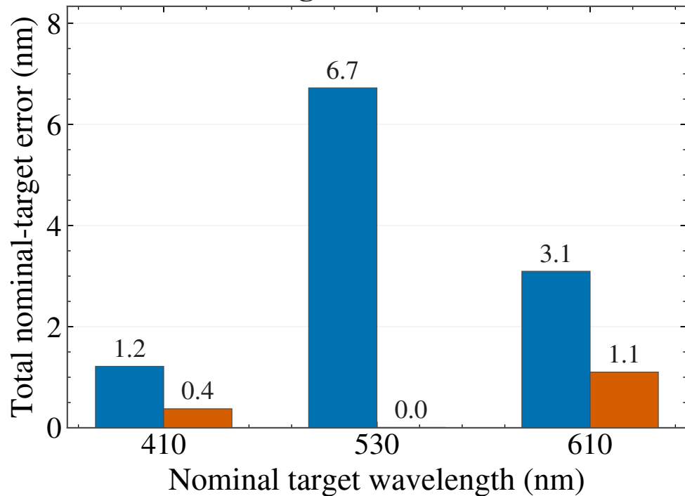
Single-notch filter
