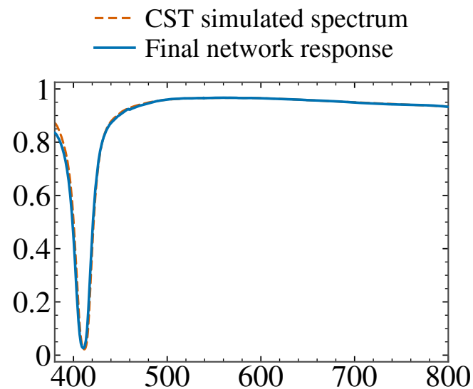
CST validation
