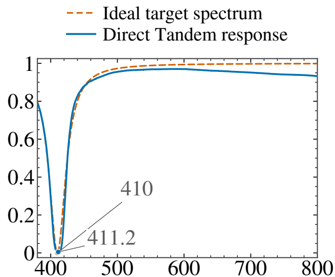
Direct Tandem
