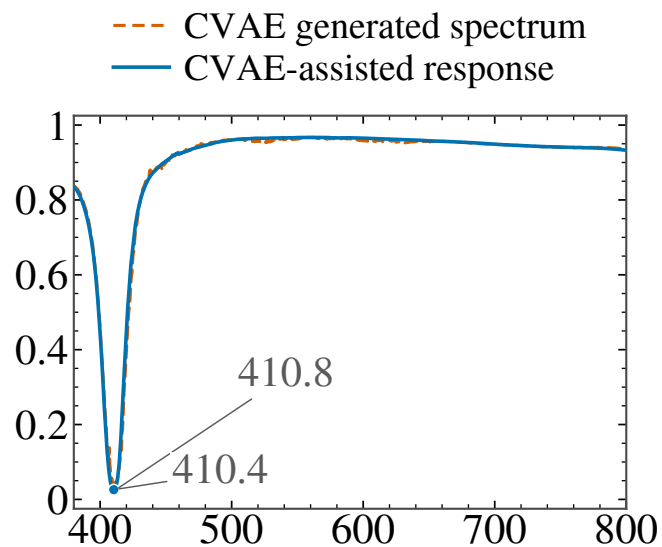
CVAE-assisted Tandem
