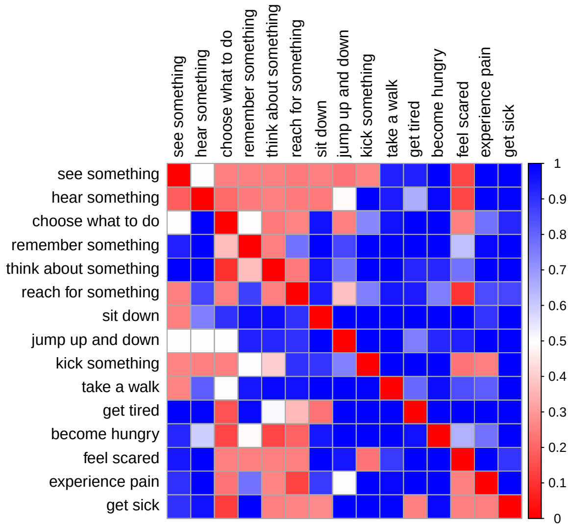
Causal RDM – subj_109
