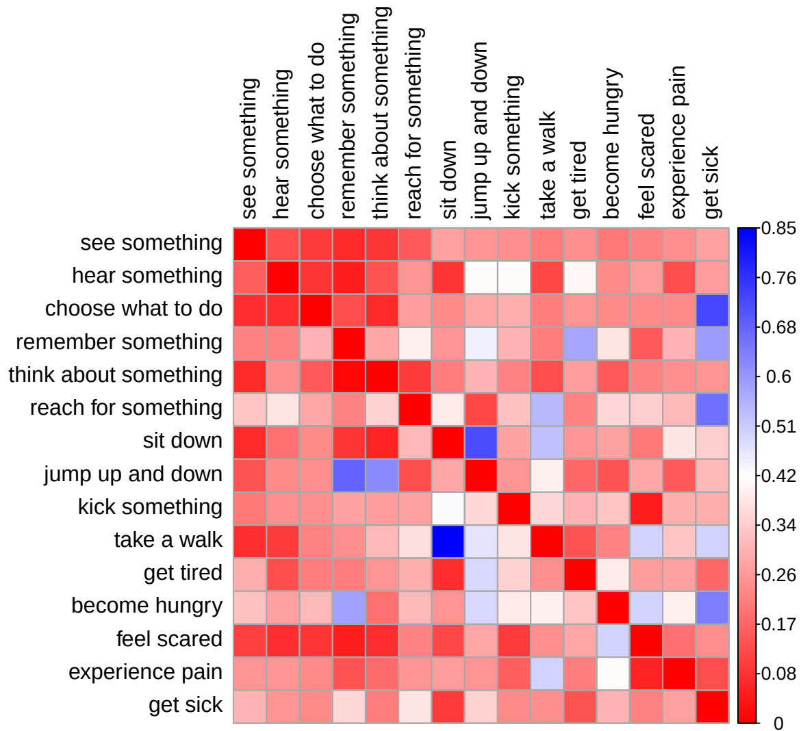
Causal RDM – subj_124
