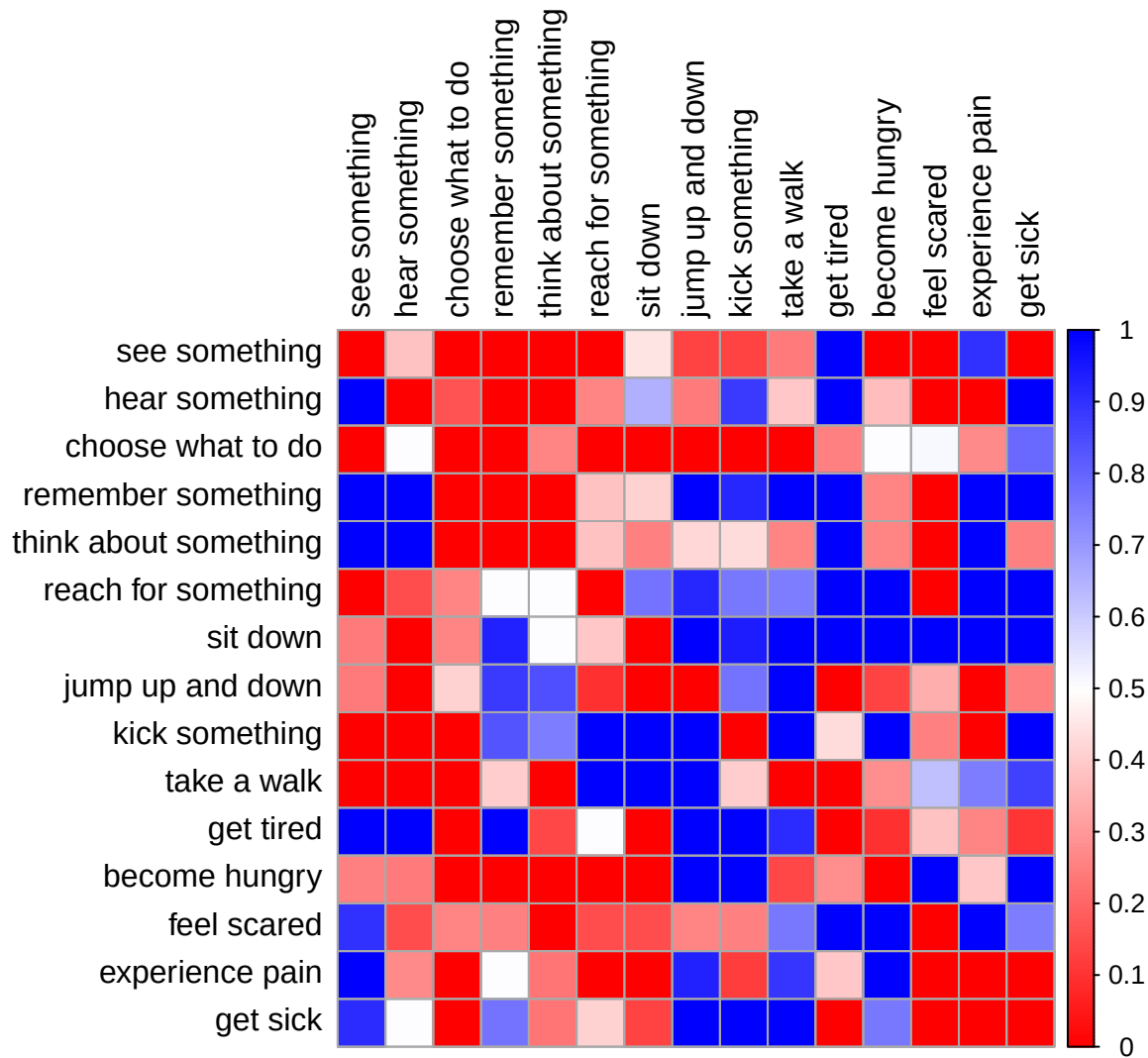
Causal RDM – subj_13
