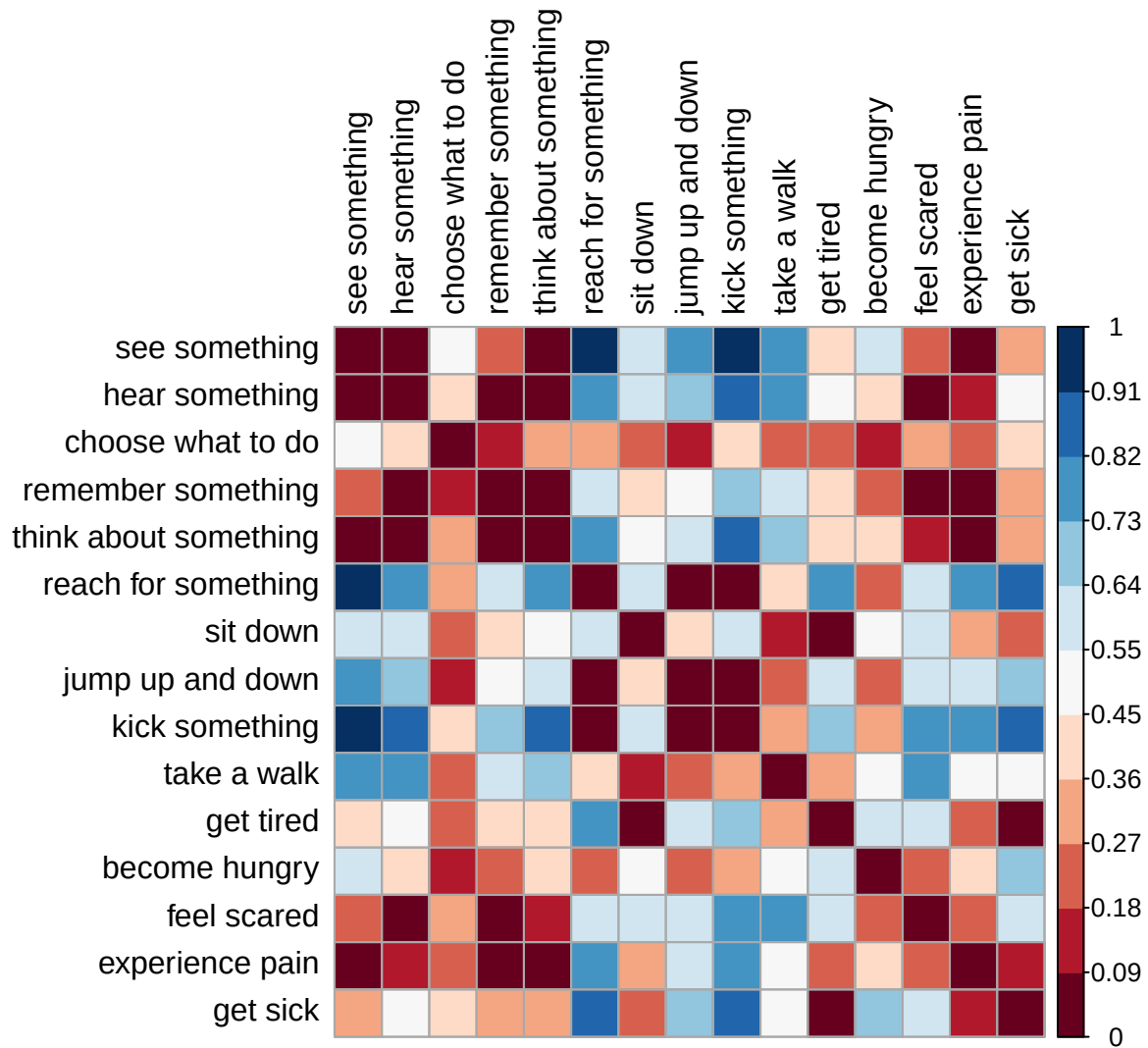
Freesort RDM – subj_06
