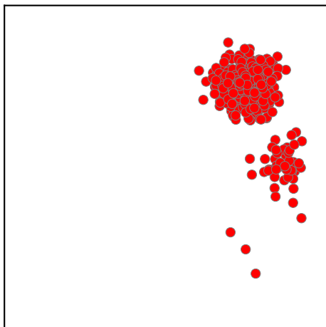
8gaussians ( \eta = 0.06 )
