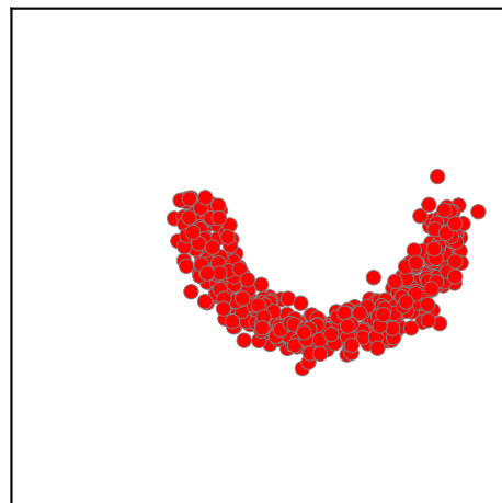
moons ( \eta = 0.06 )
