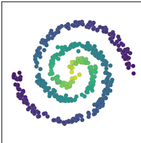
2spirals ( \eta = 0.06 )
