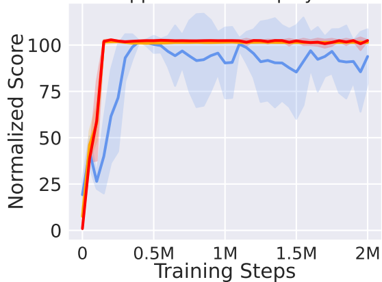
hopper-medium-replay-v2
