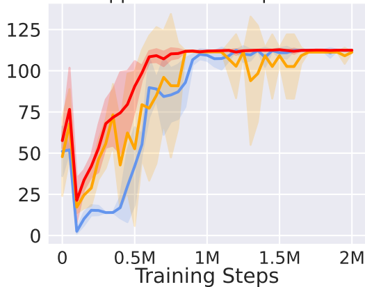
hopper-medium-expert-v2
