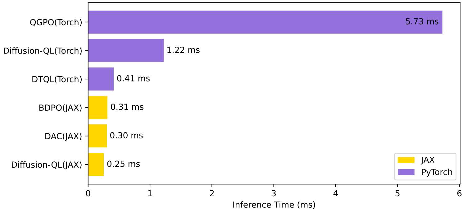
Inference Time Comparison
