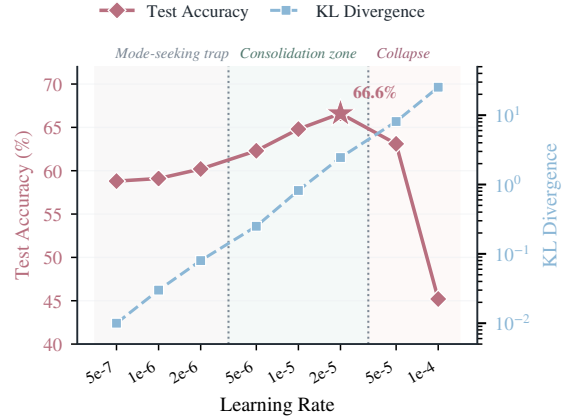
Figure 4: Phase diagram of GRPO learning rate on Medicine, revealing three regimes. Mode-seeking trap ( lr \leq 2e-6 ): accuracy stagnates, KL stays near zero. Consolidation zone ( 5e-6 to 2e-5 ): accuracy peaks at 66.6%, KL rises moderately. Collapse ( \geq 5e-5 ): KL explodes while accuracy drops sharply. The optimal lr produces a controlled 2.45 nats KL shift, enough for genuine distribution movement without catastrophic drift.
