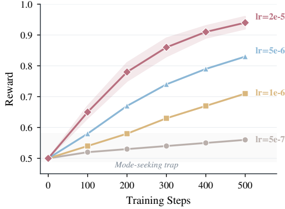
Figure 2: GRPO reward trajectories on Medicine at different learning rates. At standard lr=5e-7 (gray), reward remains trapped near initialization, the mode-seeking trap. Higher learning rates progressively escape this trap, with lr=2e-5 (rose) achieving reward 0.94 and translating to +7.4% test accuracy. Translucent band shows multi-seed variance.
