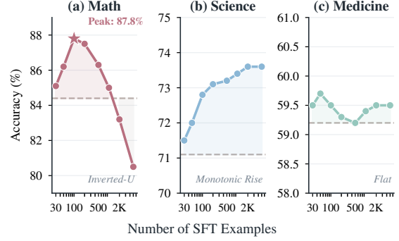
Figure 3: SFT data scaling across three domains (small multiples). Math shows a sharp inverted-U peaking at N=100 then declining below base. Science rises monotonically. Medicine remains flat regardless of data size. These three patterns correspond to high, moderate, and low base-model accuracy respectively. Full multi-seed results in Appendix F.
