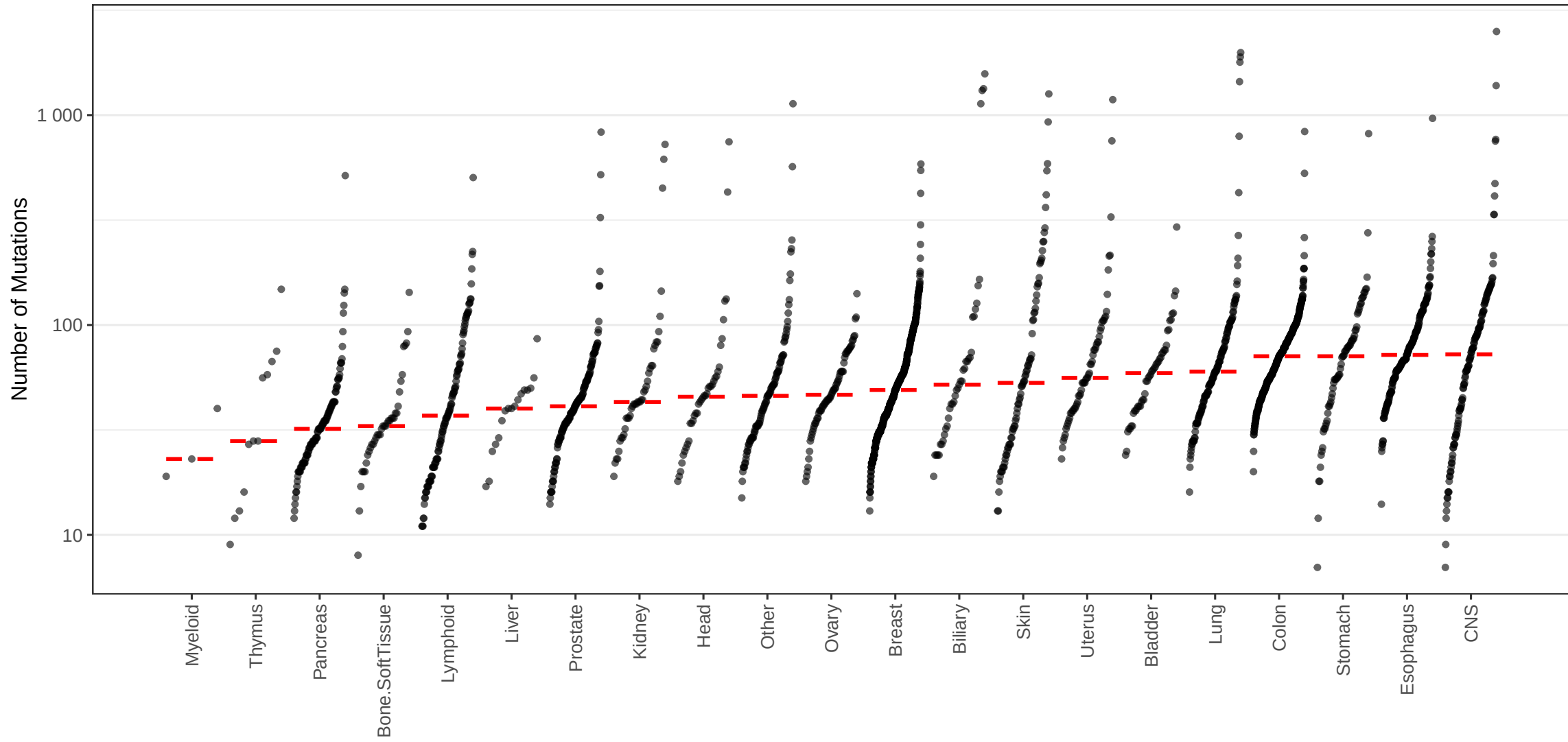
C_ID4 mutations
