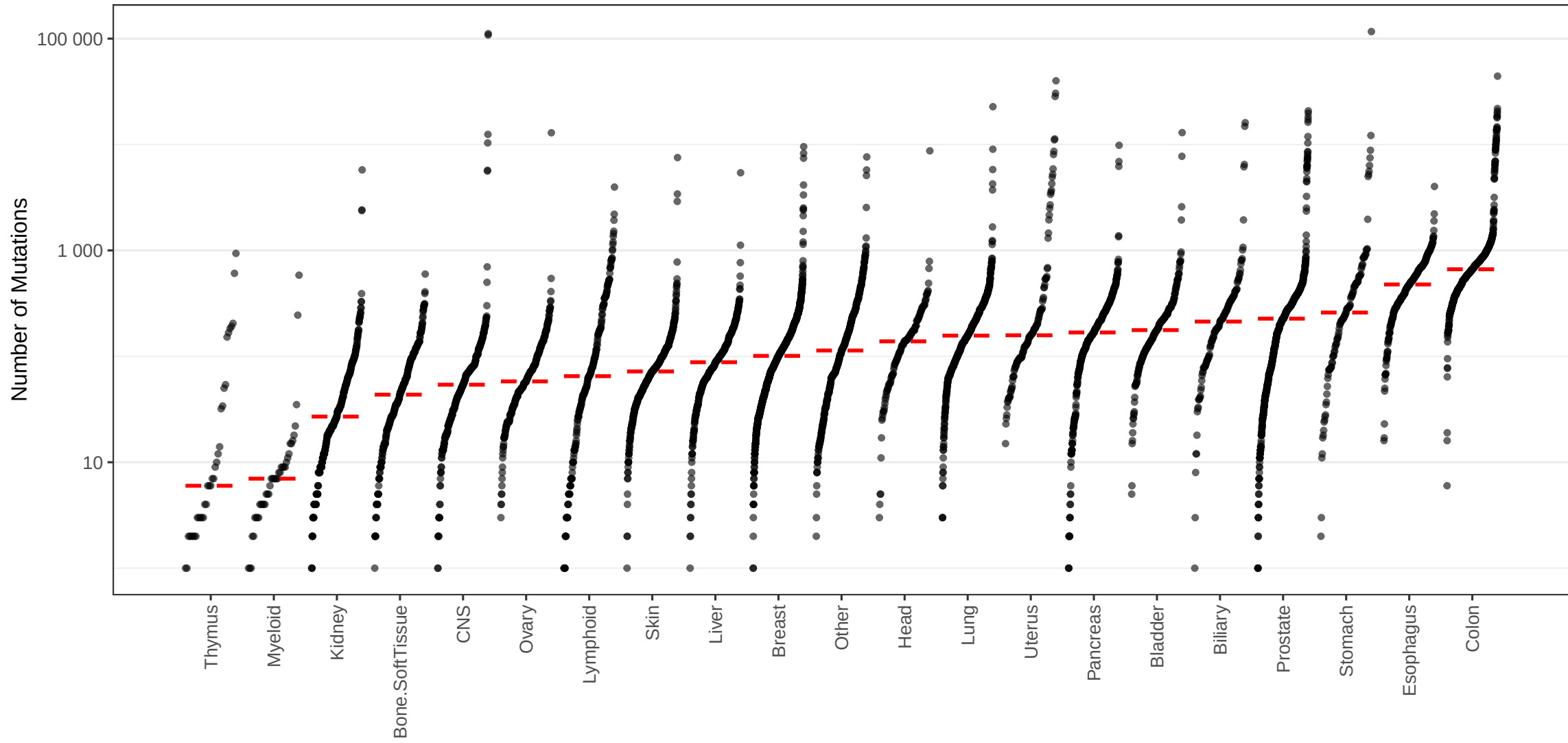
C_ID1 mutations
