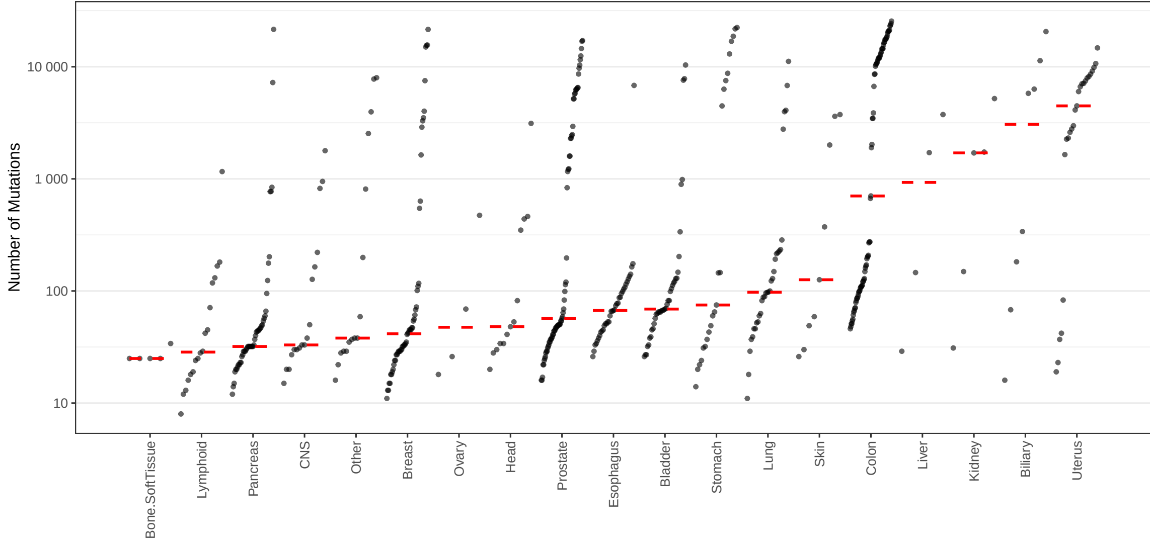
C_ID7 mutations
