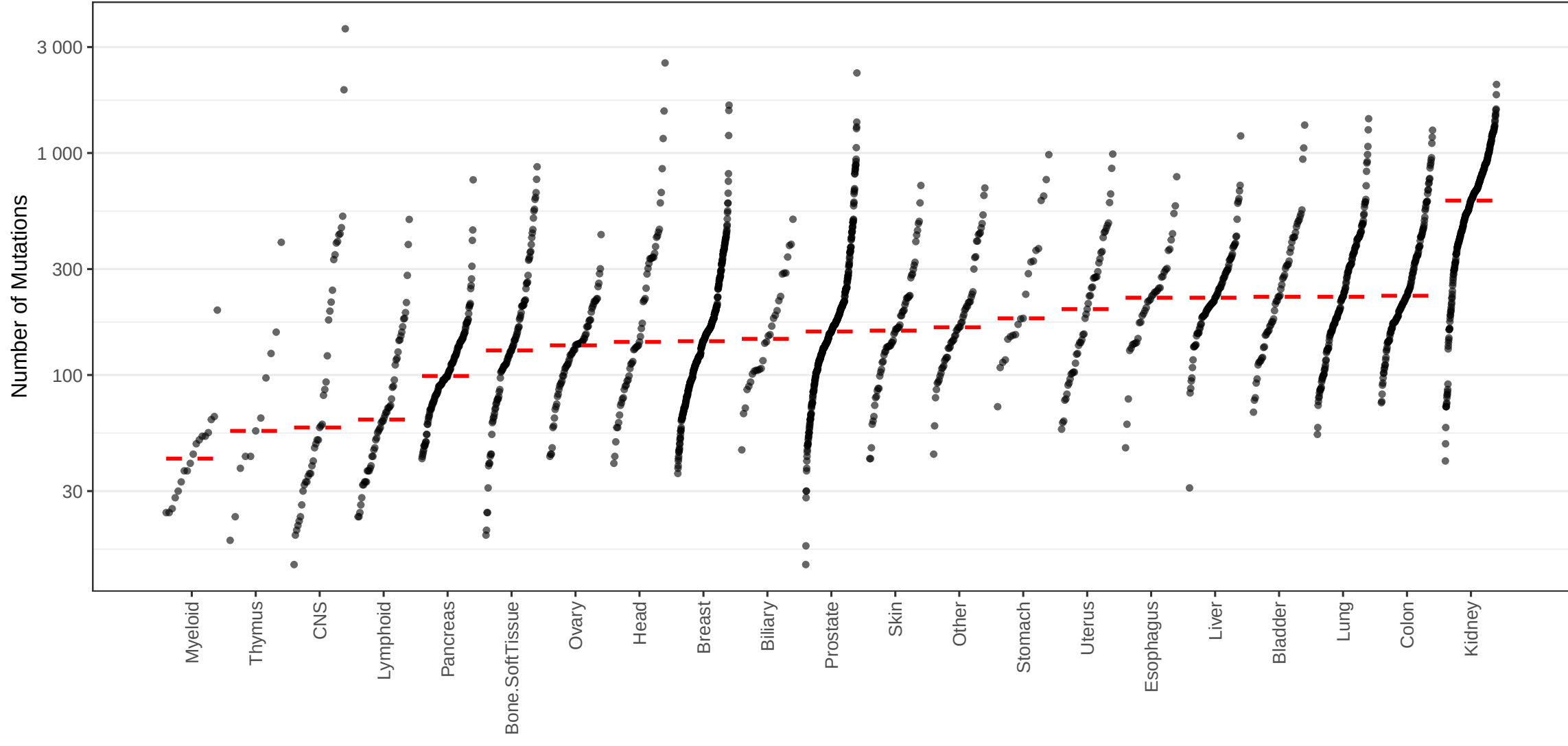
C_ID5 mutations
