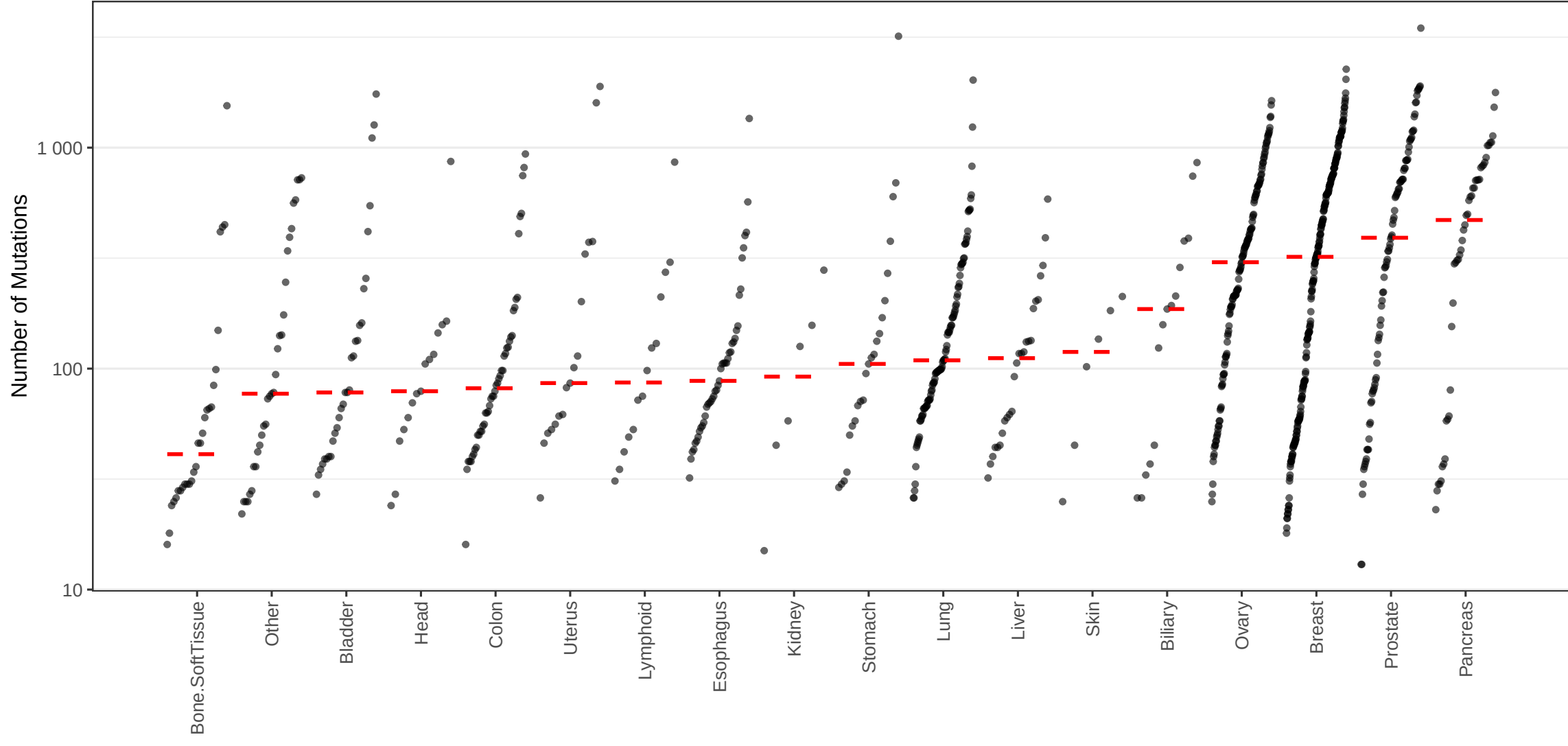
C_ID6 mutations
