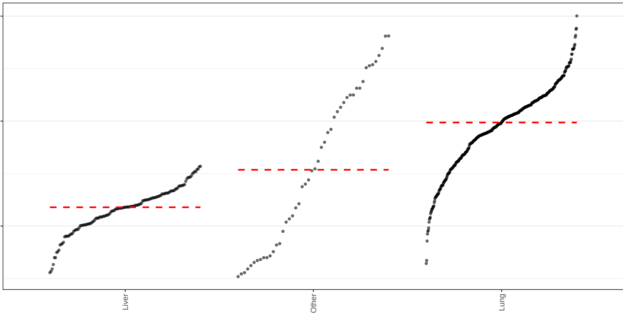
C_ID3 mutations
