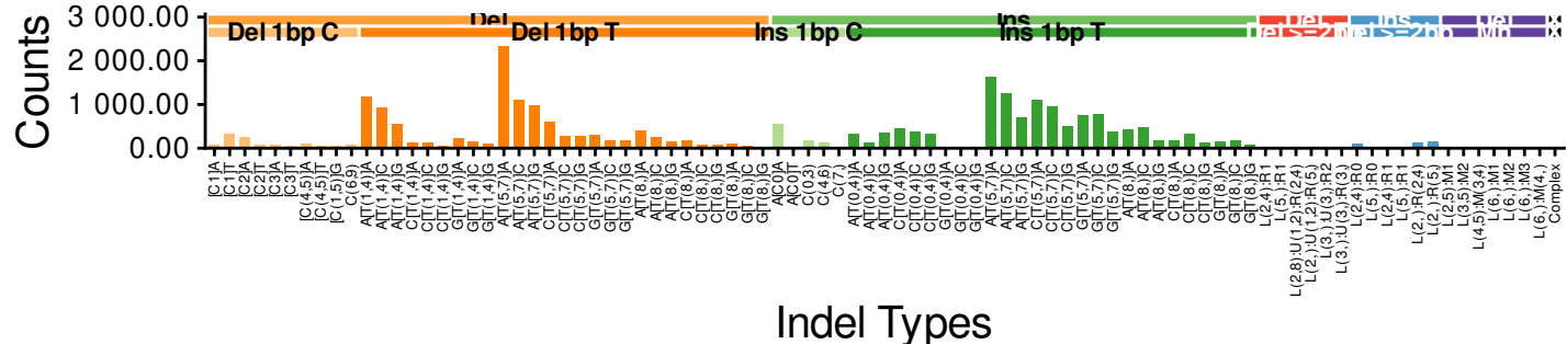
Colon::SP17905 cosine to Koh = 0.952211666463103
