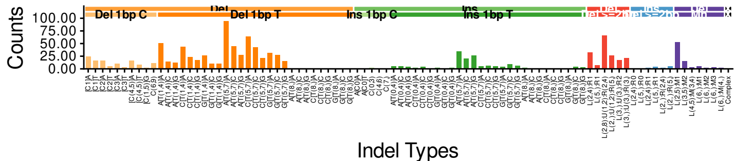
Koh ID InD20 cosine to extracted = 0.660100328823997
