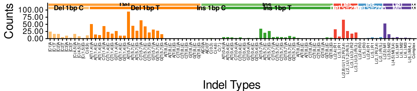
Current exemplar Prostate::SP112817 cosine to sig = 0.984695082908958
