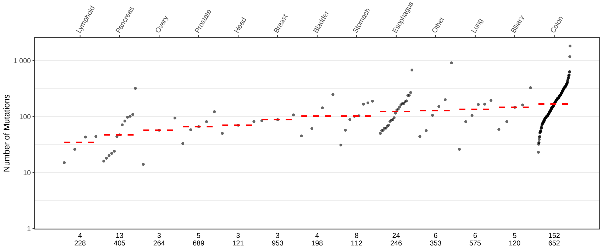
C_ID14 mutations
