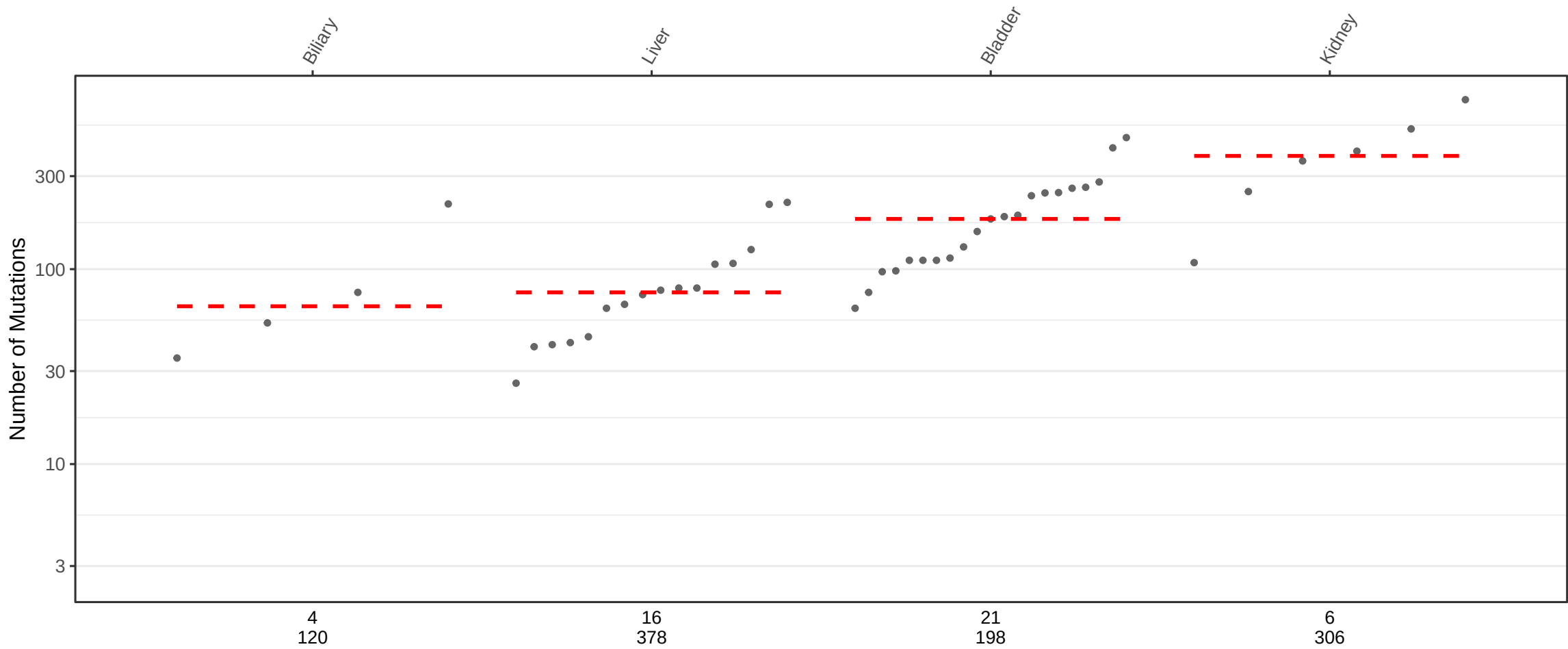
C_ID23 mutations
