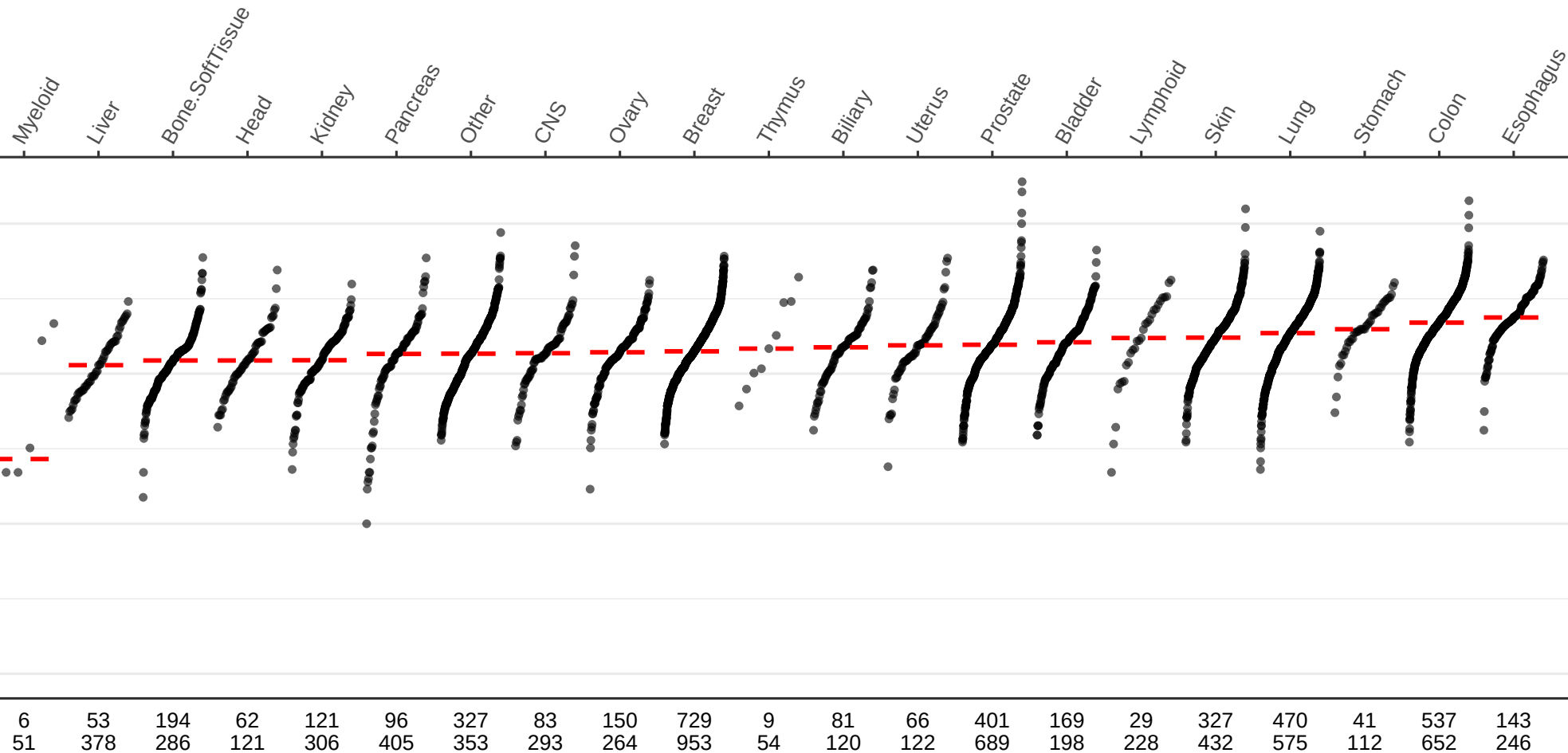
C_ID19 mutations
