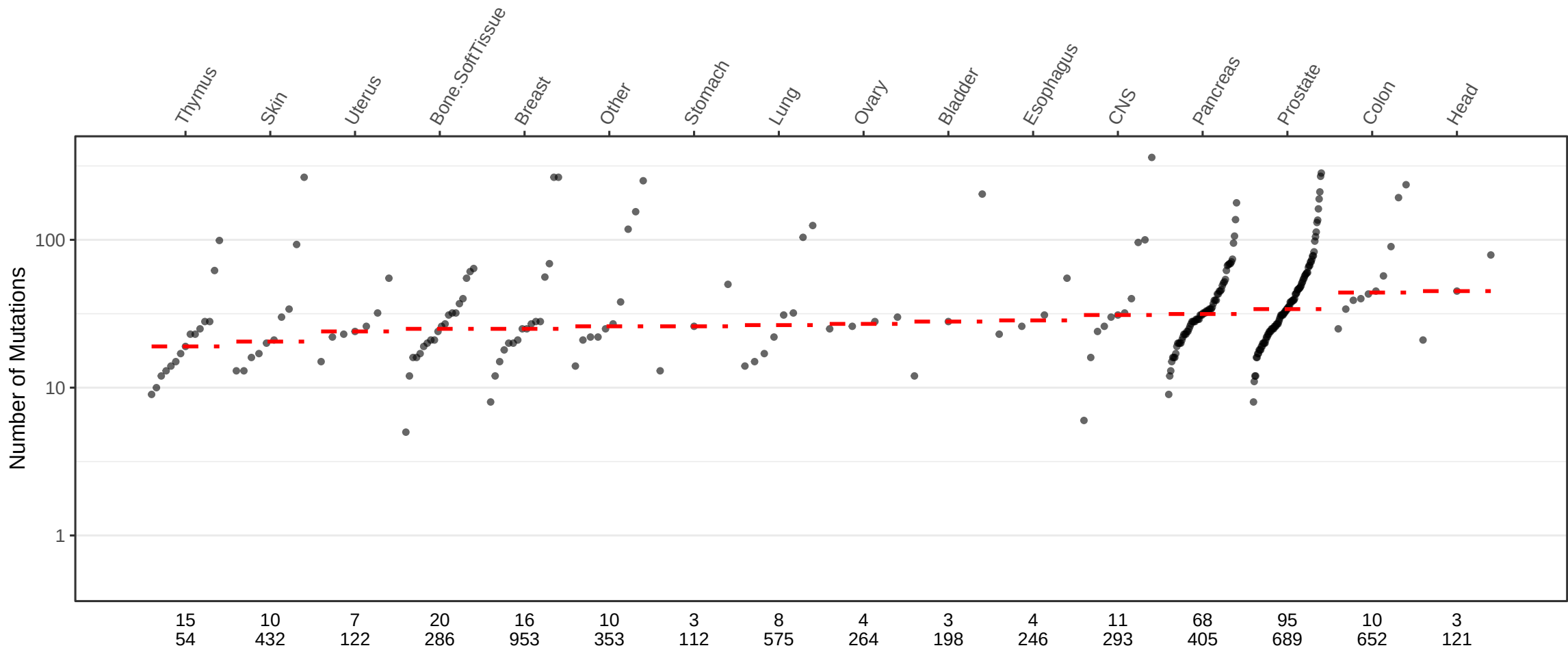
C_ID12 mutations
