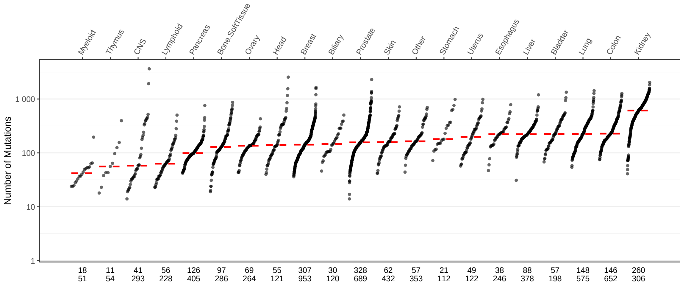
C_ID5 mutations
