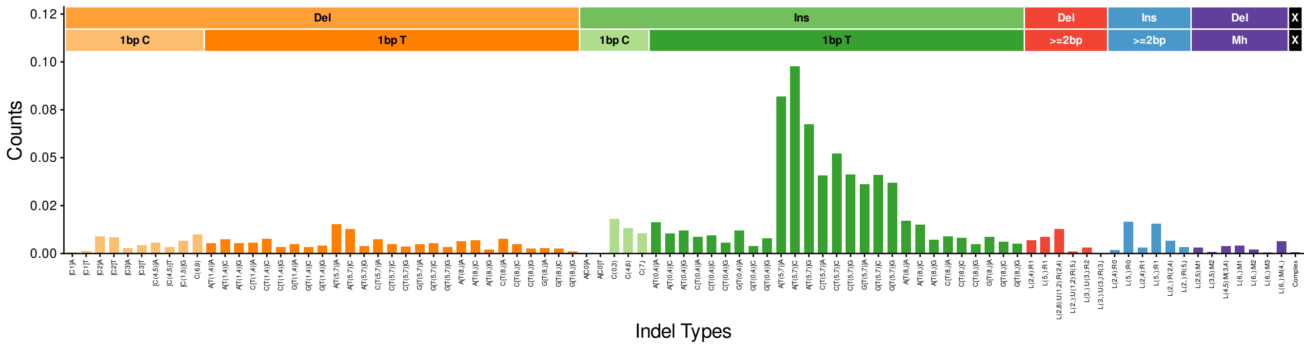
InsDel1c (cosine: 0.9365)
