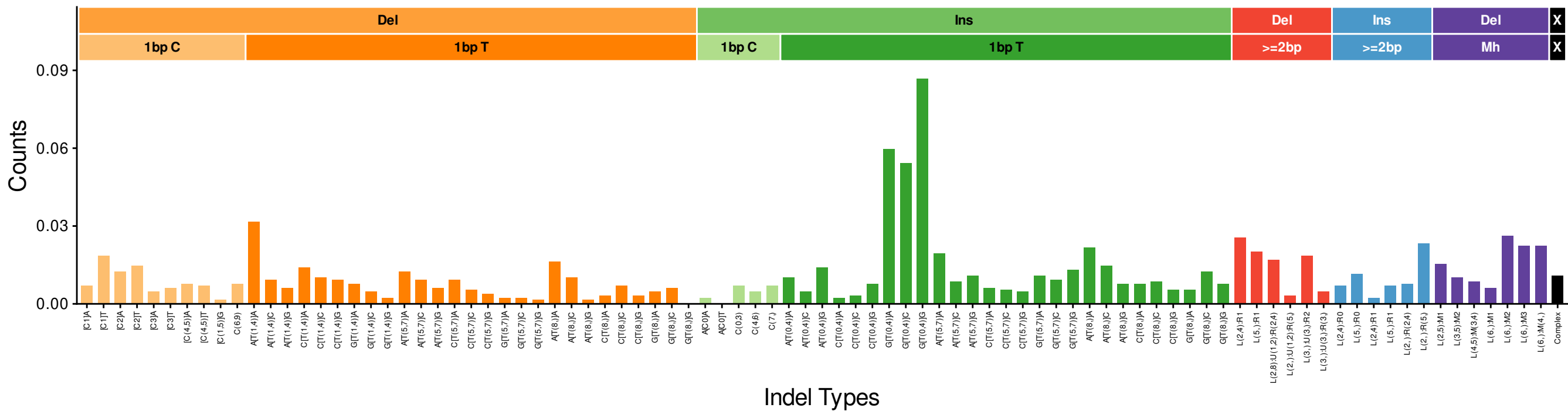
InD32
