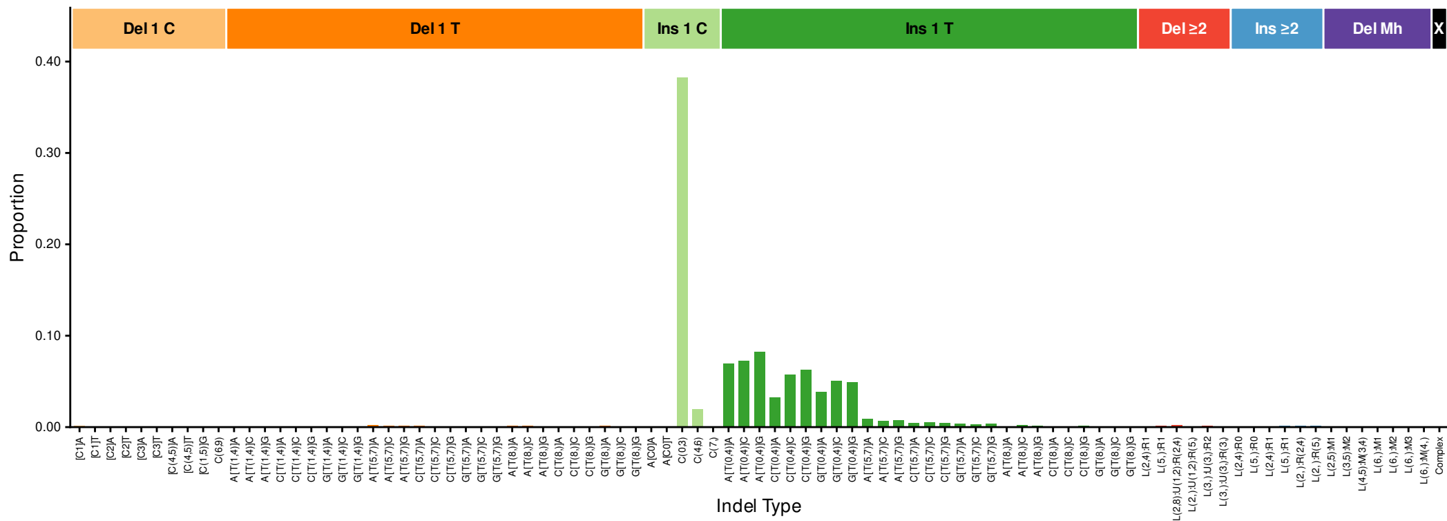
InsDel11 (cosine = 0.965)
