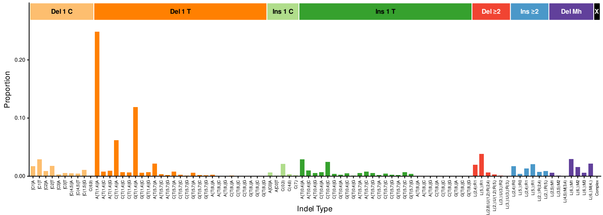
InsDel13 (cosine = 0.935)
