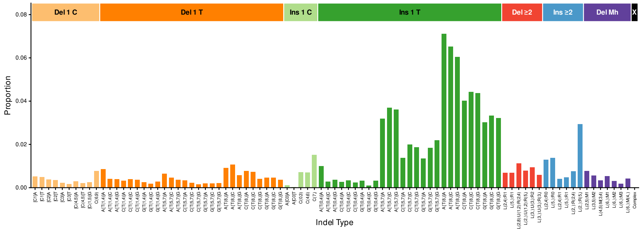
InsDel1a (cosine = 0.911)
