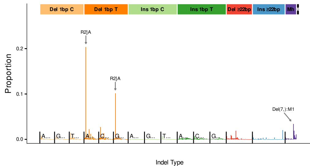
InsDel13 (476-type)
