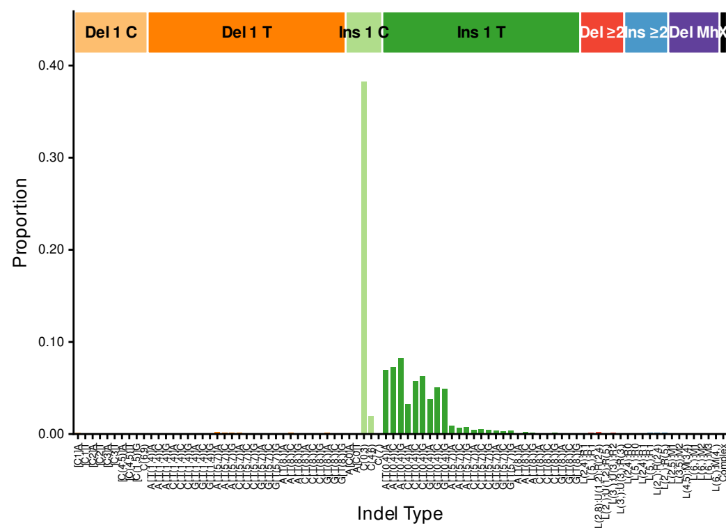
InsDel11 (476-type)
