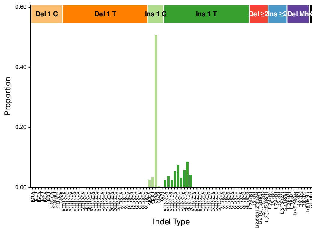
InsDel16 (476-type)
