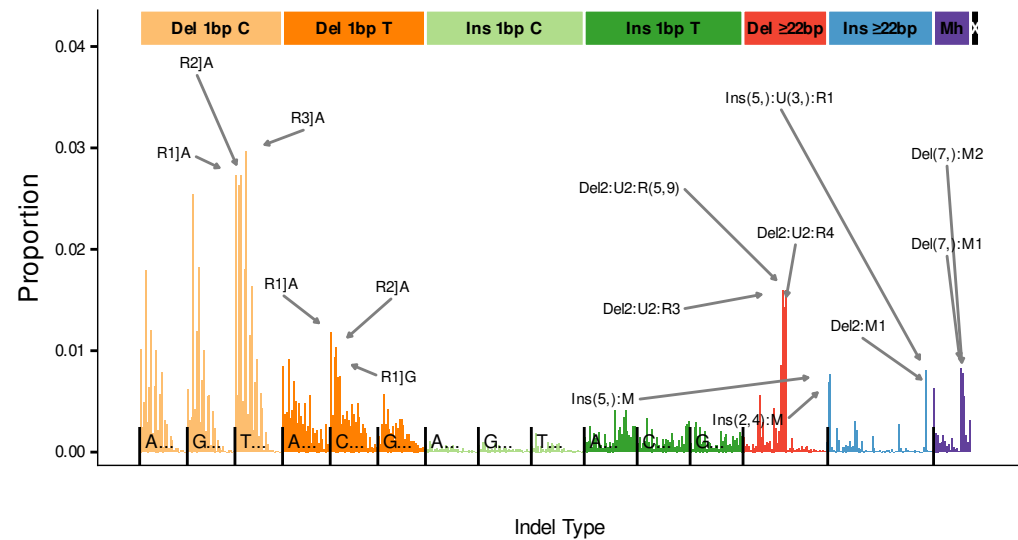
InsDel3a (476-type)
