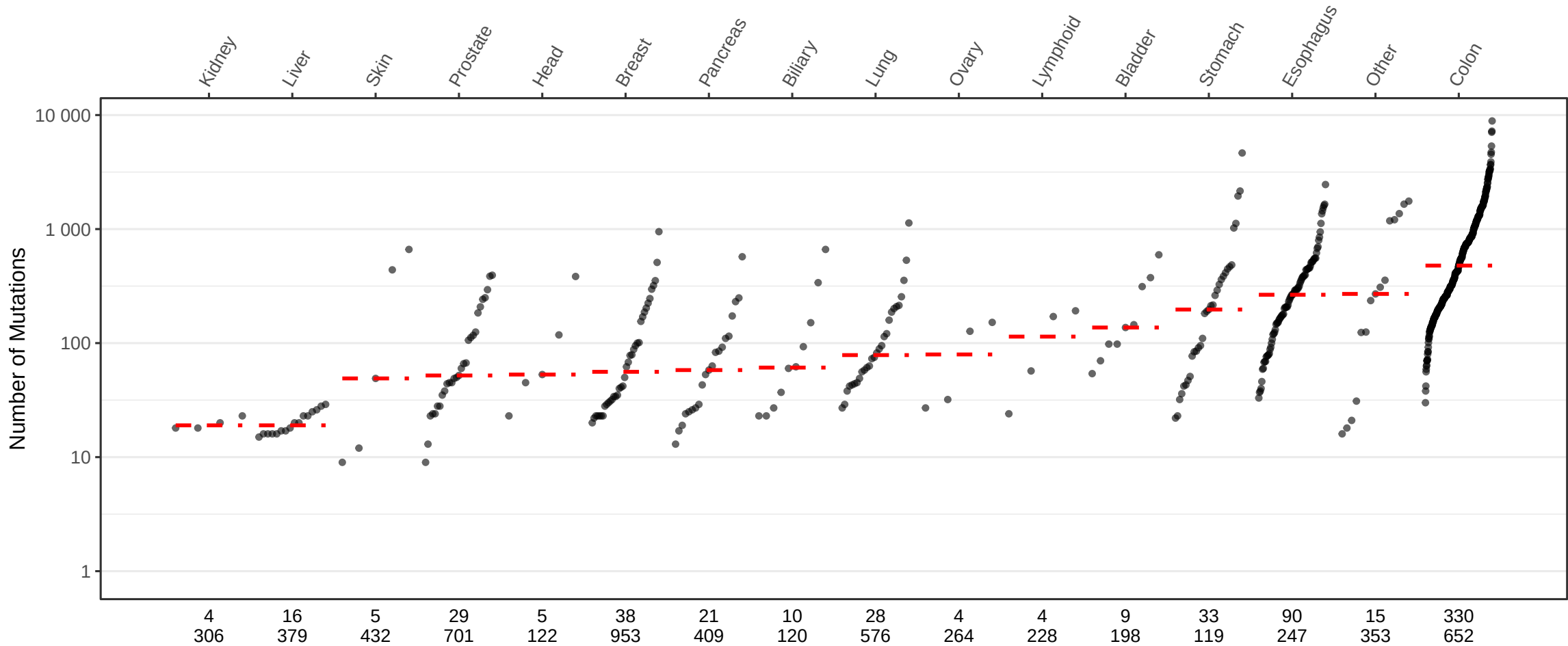
InsDel_D mutations
