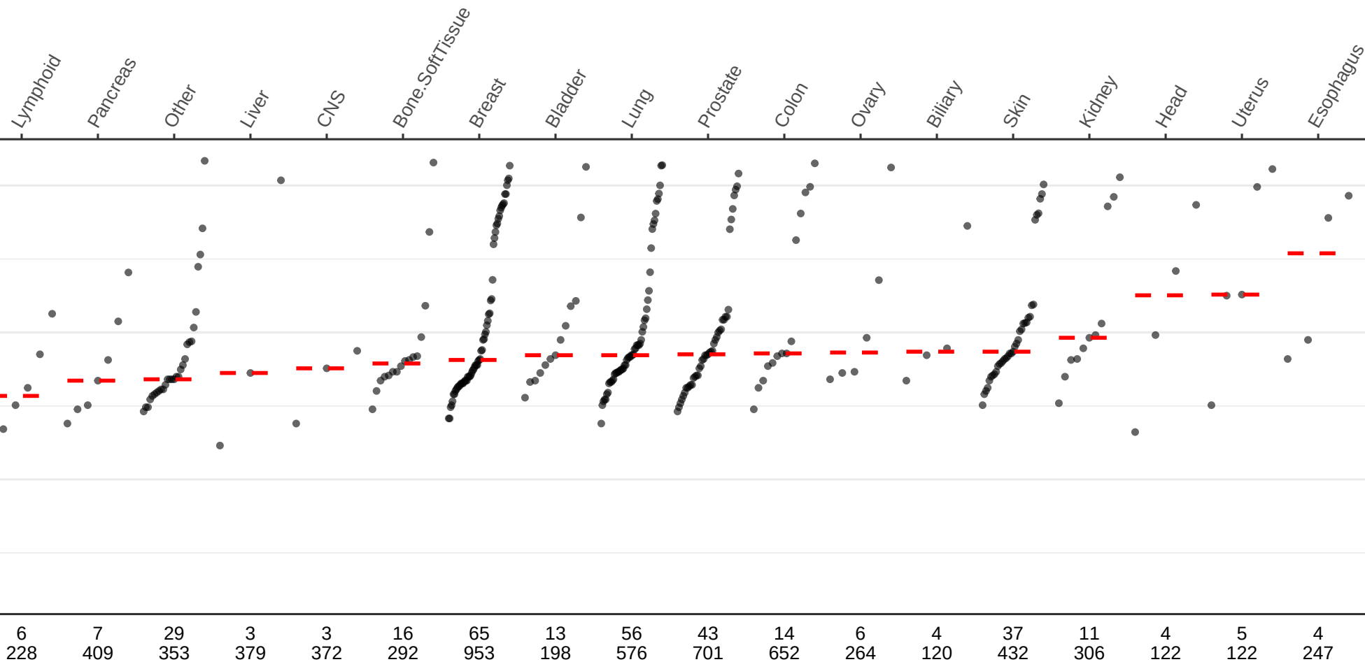
InsDel_E mutations
