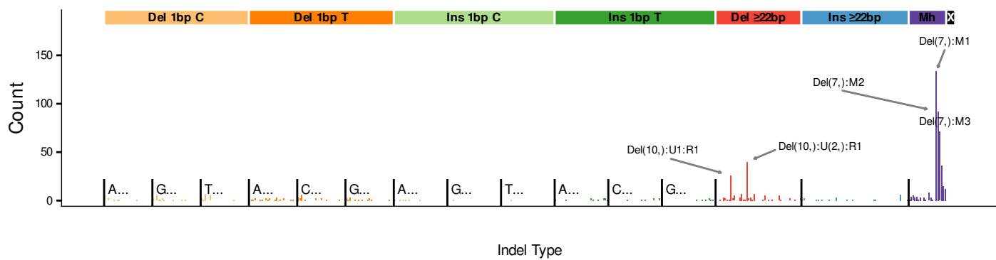
Breast::SP116365 (table 1 type-89 exemplar)
