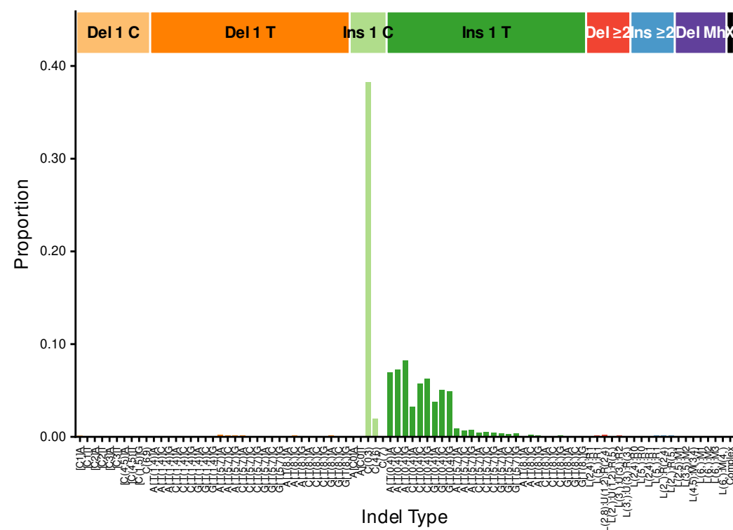
InsDel11 (89-type, cosine = 0.965)
