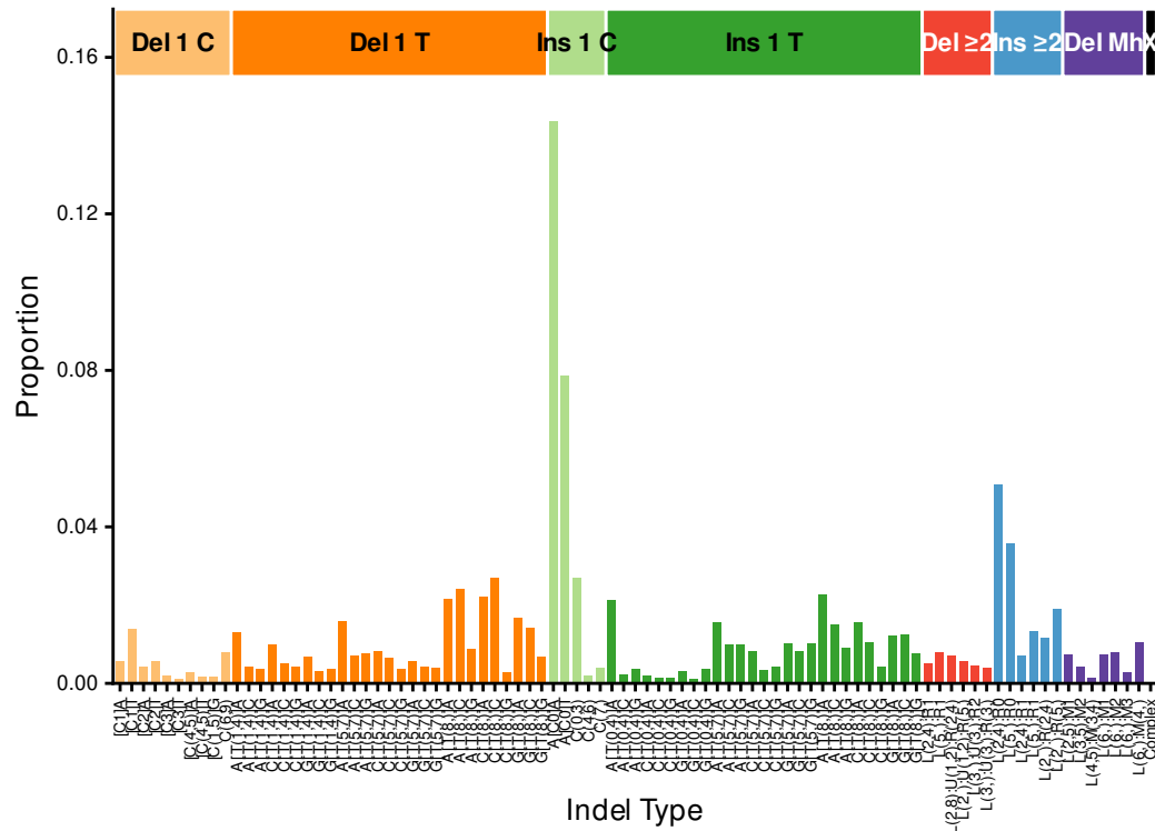
InsDel14 (476-type)
