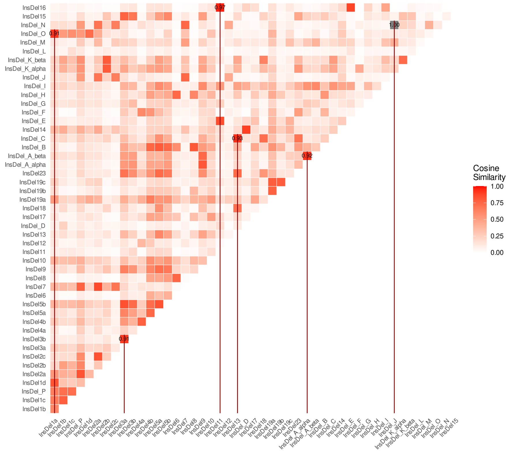
Pairwise Cosine Similarities (89-type)
