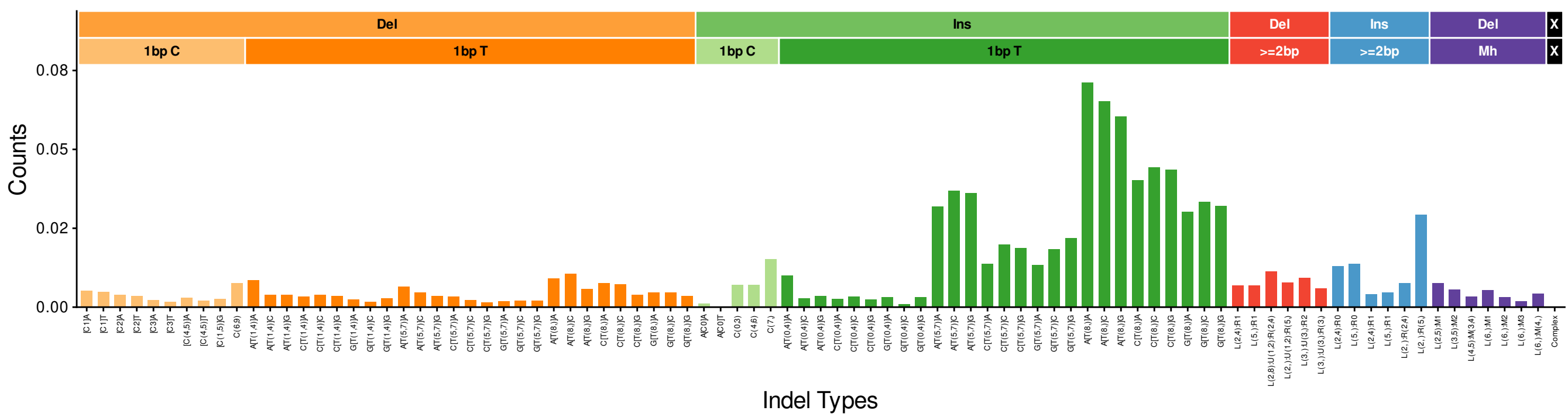
InD1 (cosine: 0.9825)
