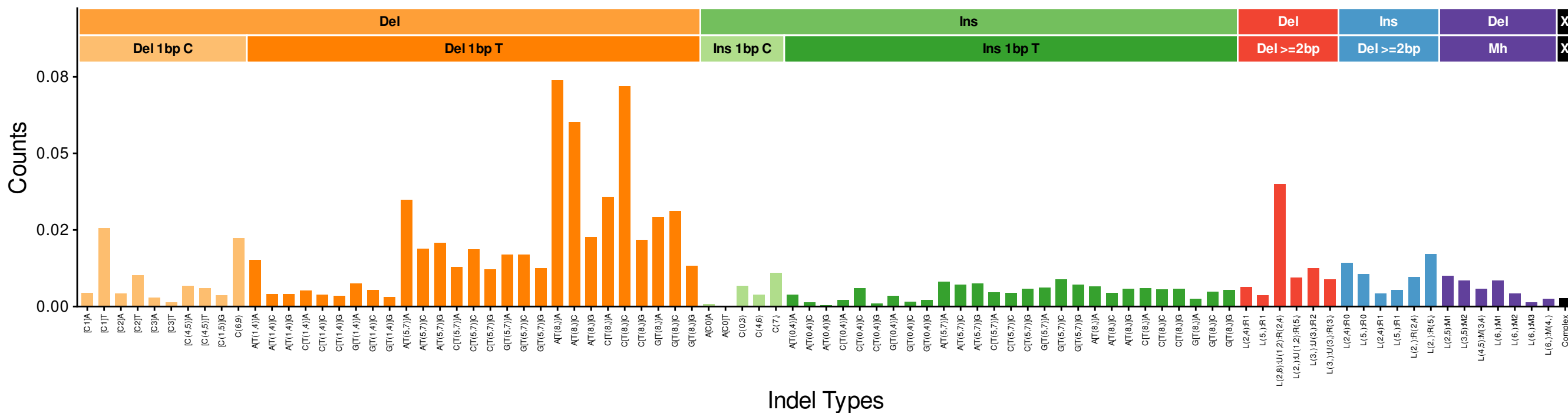
Skin..WIDE01010381T (cosine: 0.9470)
