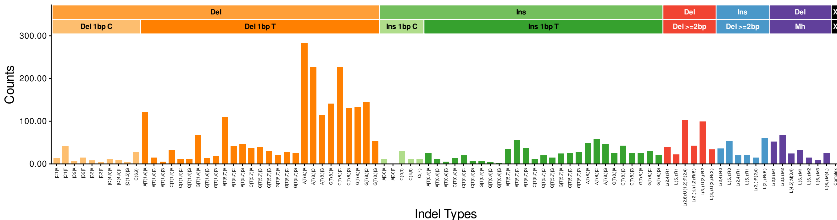
Skin..WIDE01010381T (euclidean: 0.0540)
