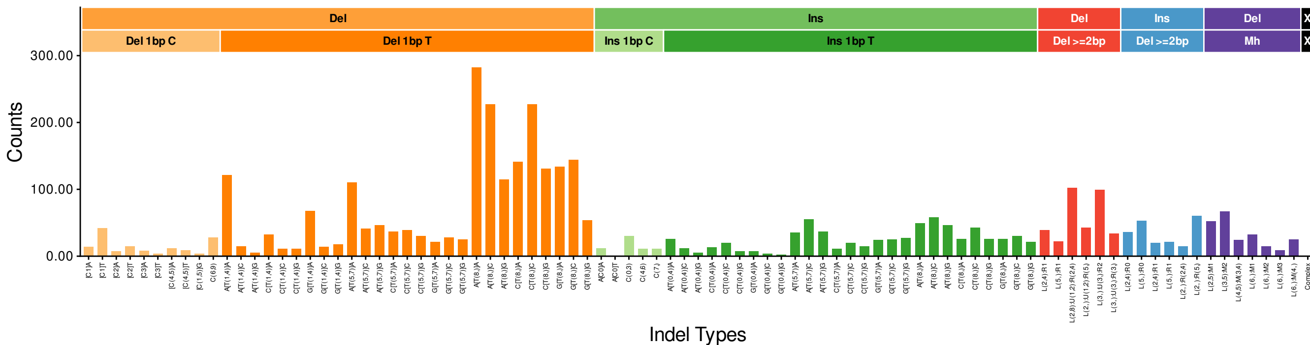
Skin..WIDE01010381T (euclidean: 0.0540)
