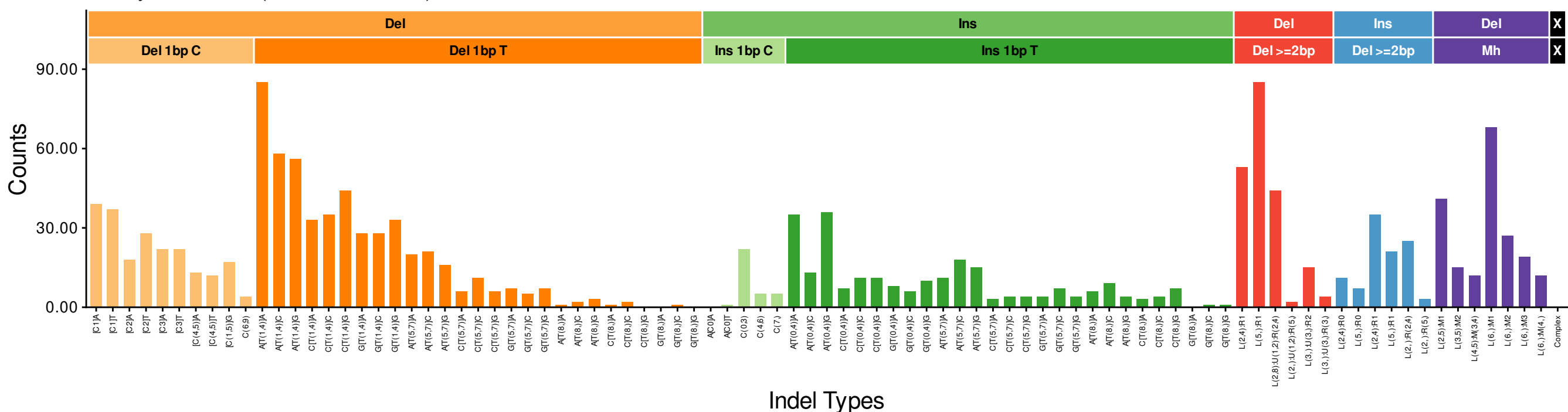
Kidney..SP102795 (euclidean: 0.0472)
