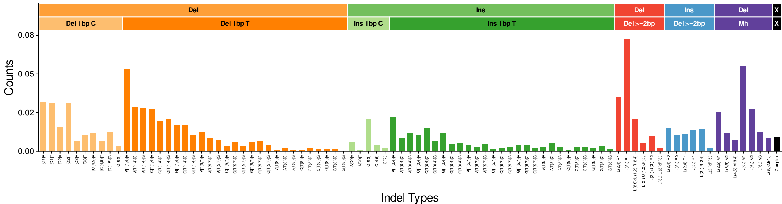
Kidney..SP102795 (cosine: 0.9558)
