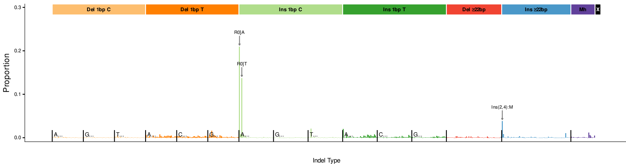
InsDel14 (cosine = 0.993)
