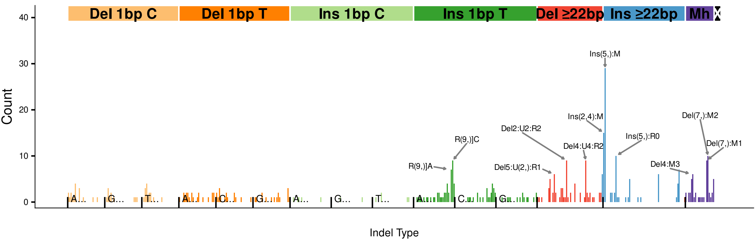
Bone.SoftTissue..CPCT02010408T (cosine: 0.9038)
