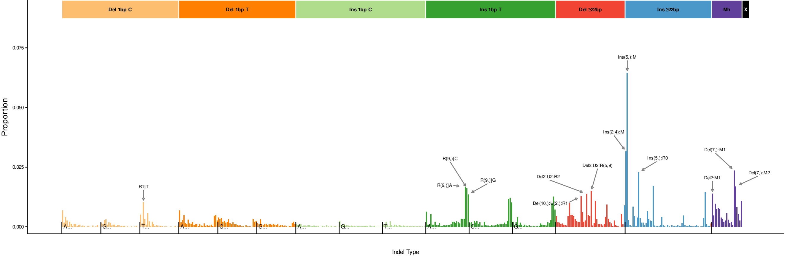
InsDel19a
