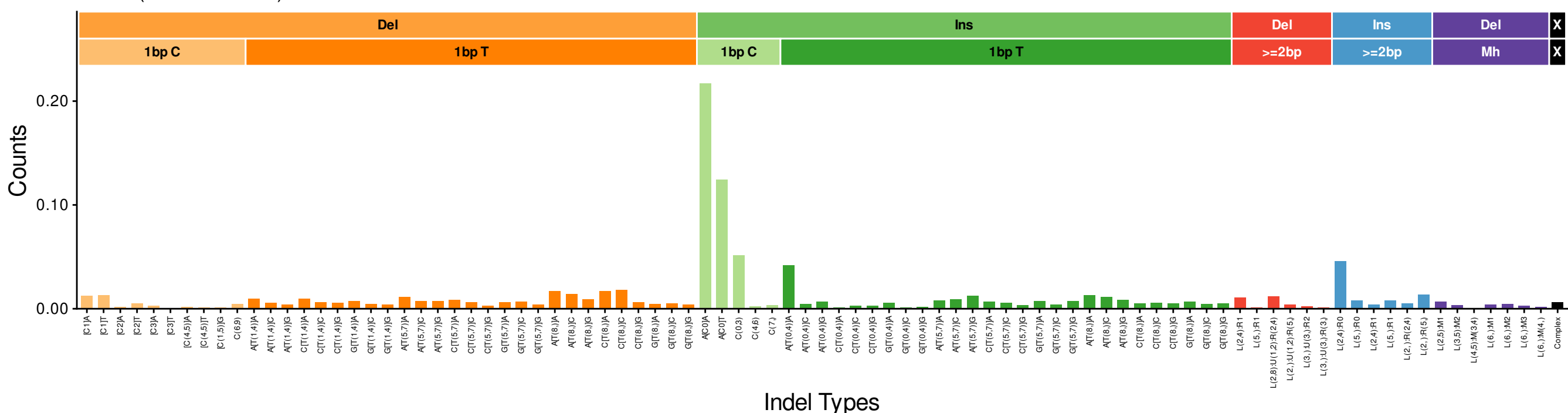
InD12 (cosine: 0.9491)
