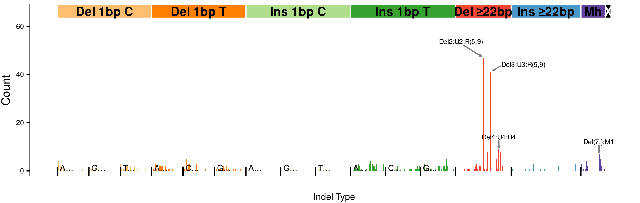
Prostate..SP112947 (cosine: 0.9577)
