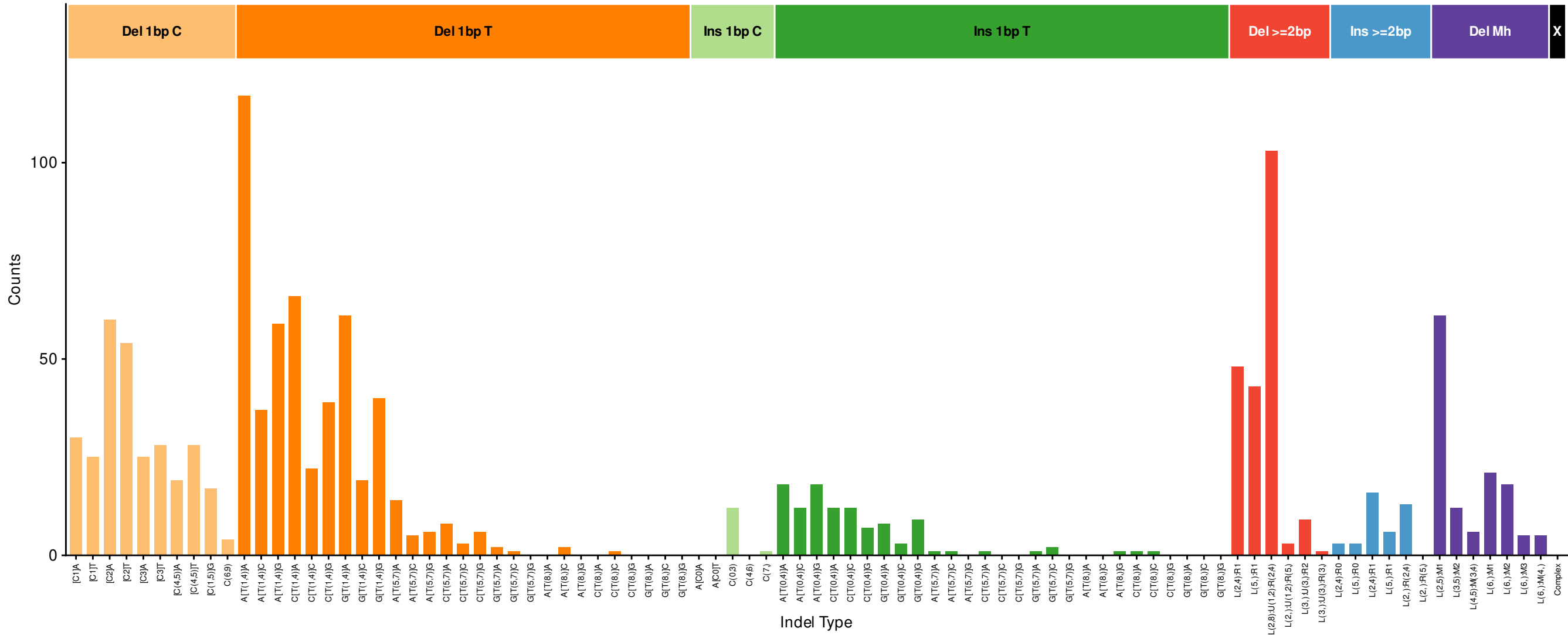
Kidney..SP102957 (cosine: 0.9606)
