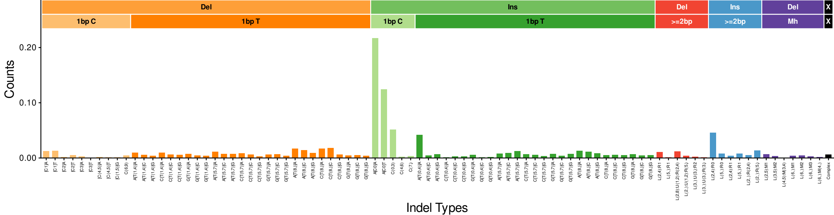
InsDel14 (cosine: 0.9803)
