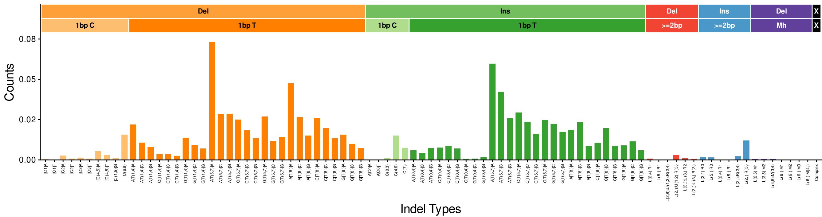
InsDel1d (cosine: 0.9073)
