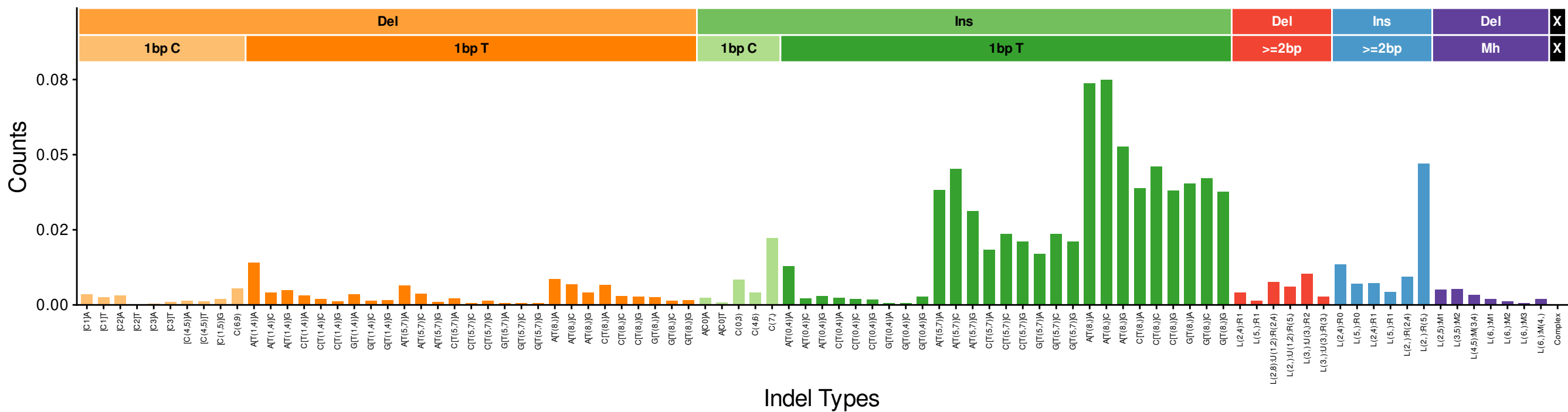
InsDel1a (cosine: 0.9825)
