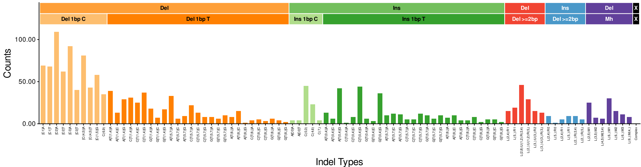
Lung..SP58101 (euclidean: 0.0509)
