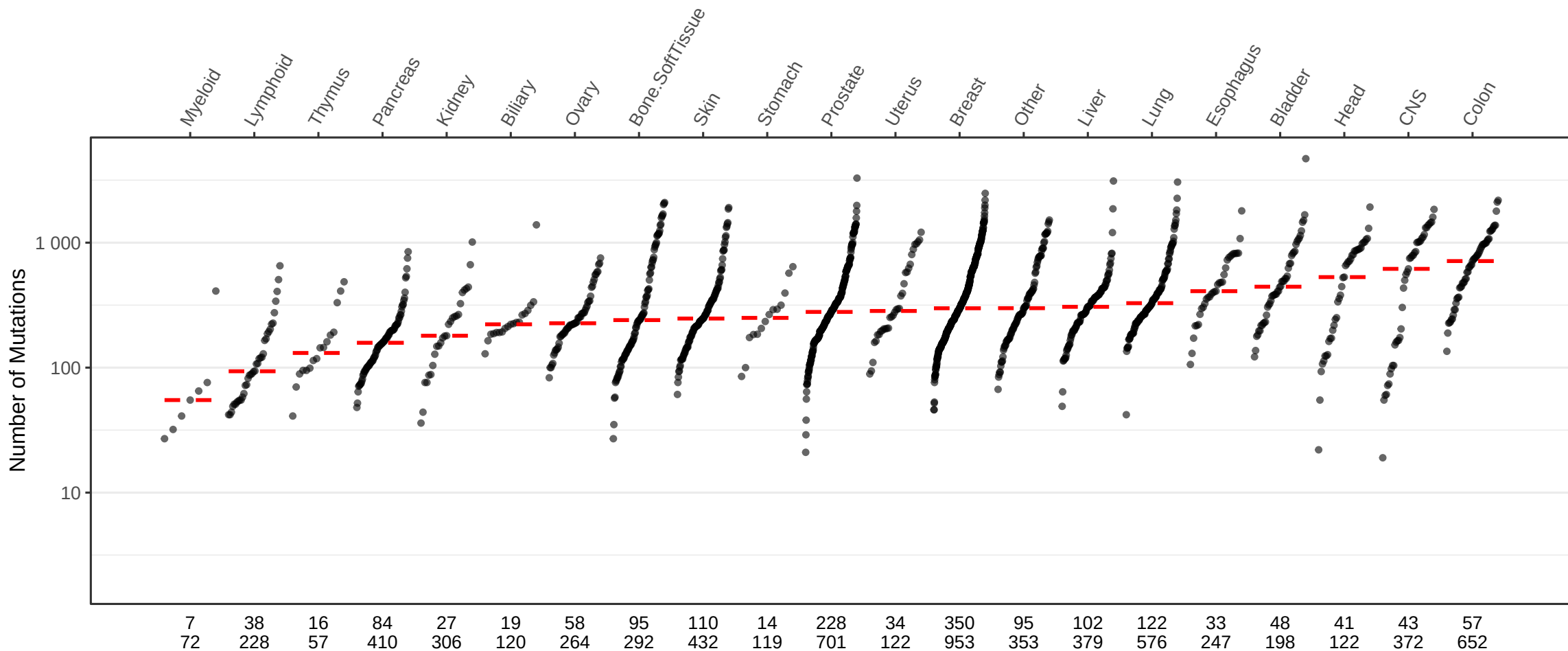
InsDel_B mutations
