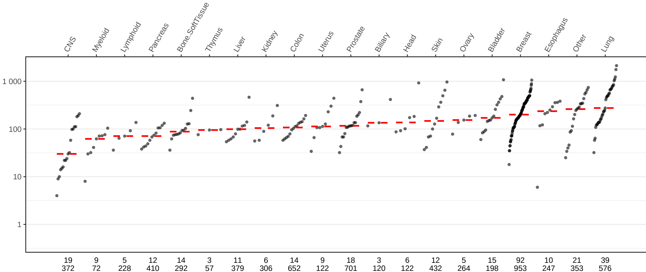
InsDel_A_beta mutations
