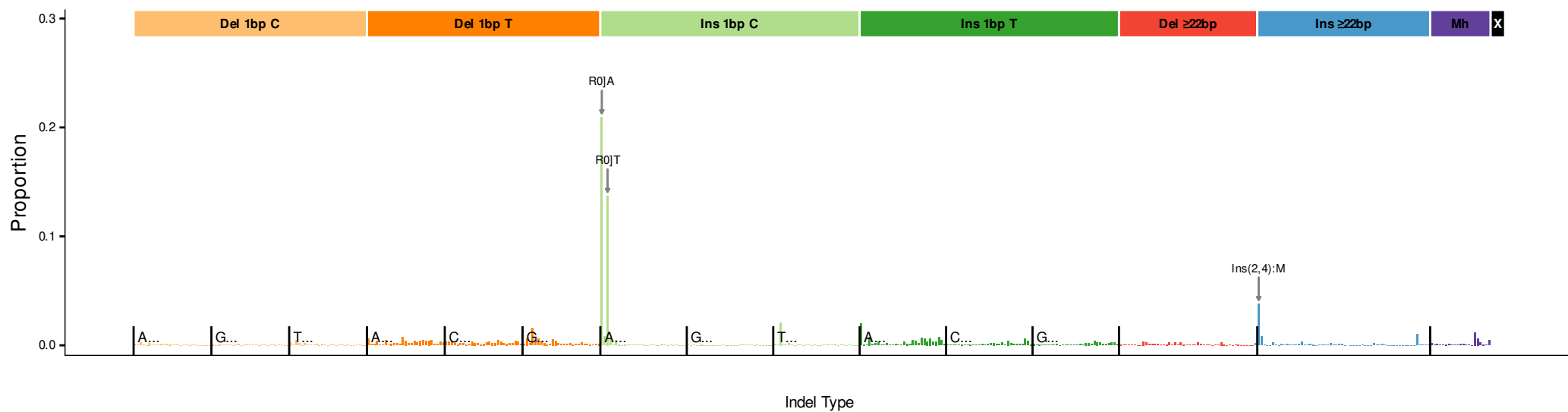
InsDel14 (cosine = 0.993)
