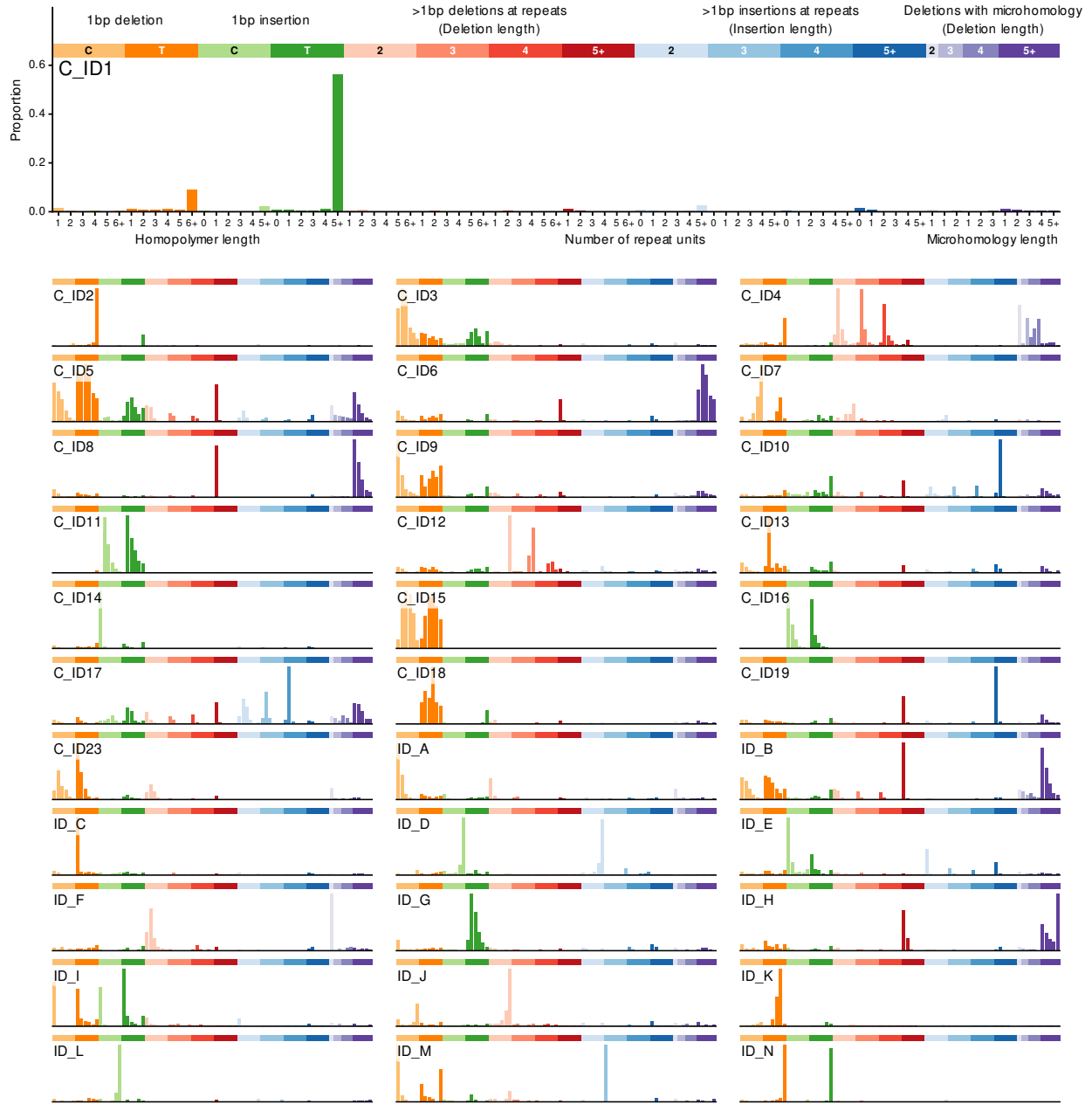
Figure 2: Profiles of signatures extracted in the 83-type classification scheme
