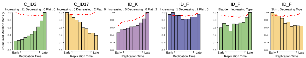
Figure 5: 83-type mutational signatures asymmetries in strands, replication timing and DNA regions.
