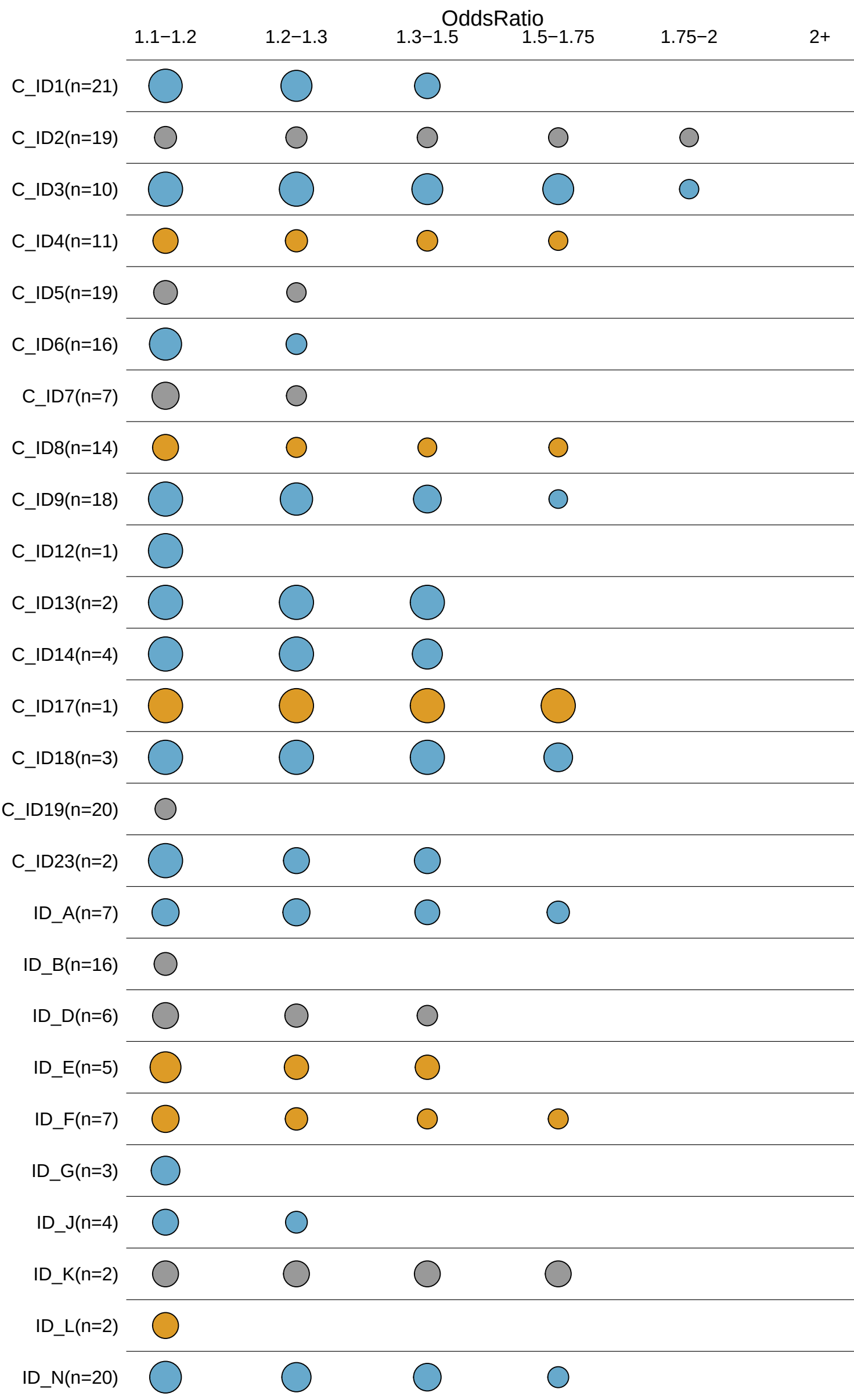
Replicational Strand Asymmetry
