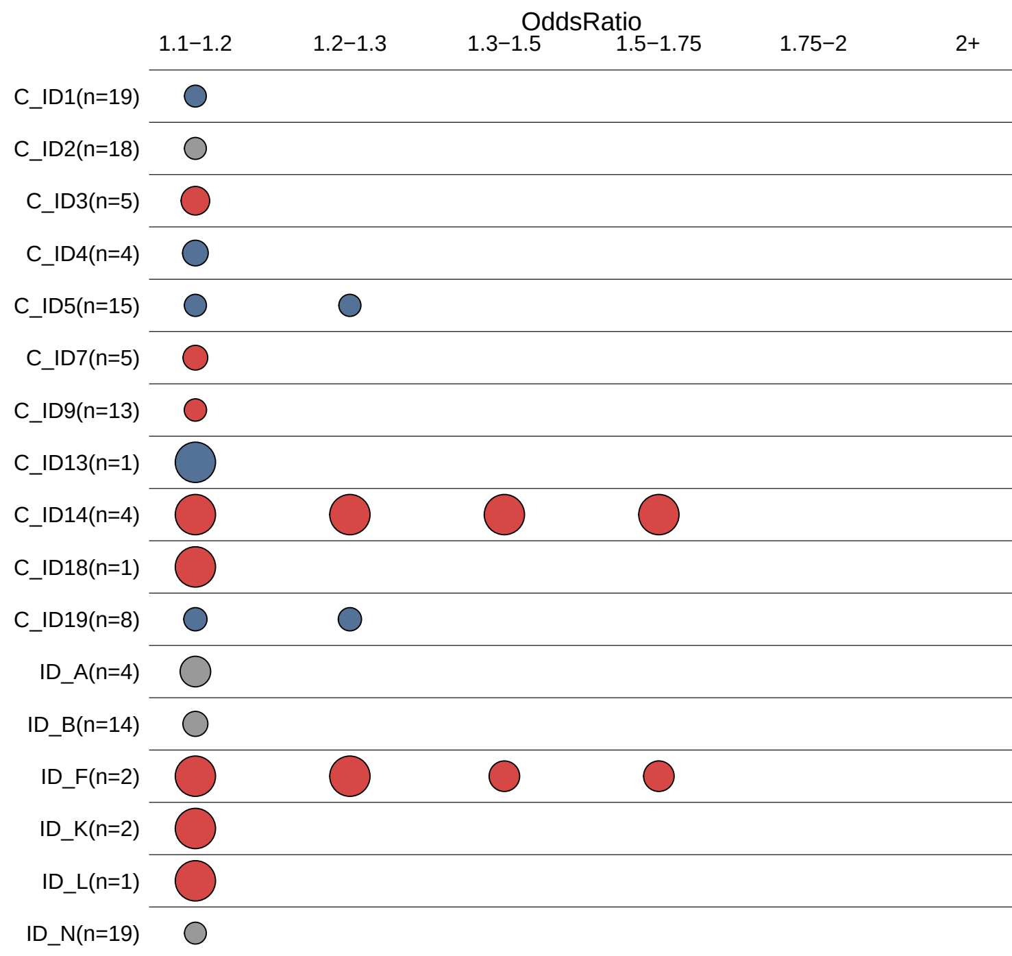
B Replication strand asymmetry
