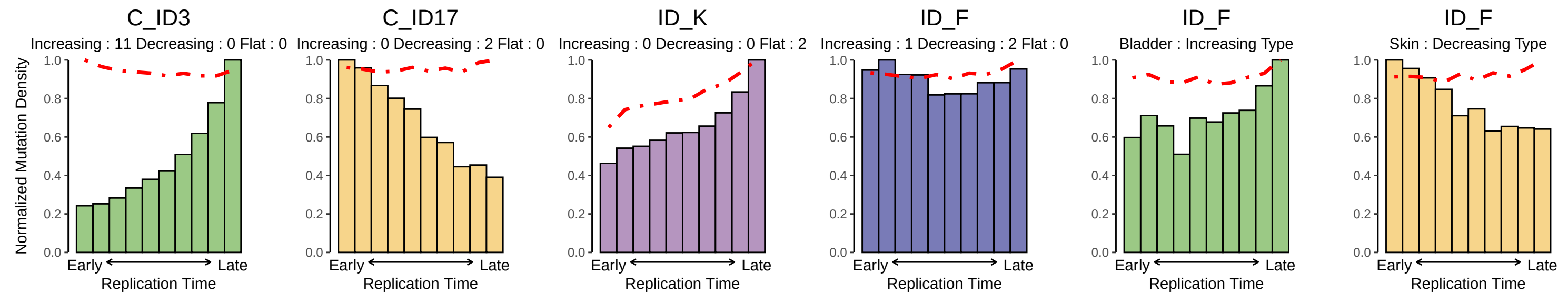
D Replication timing
