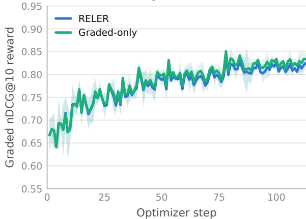
(a) Graded training reward
