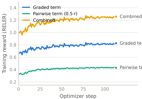
(b) RELER reward components
