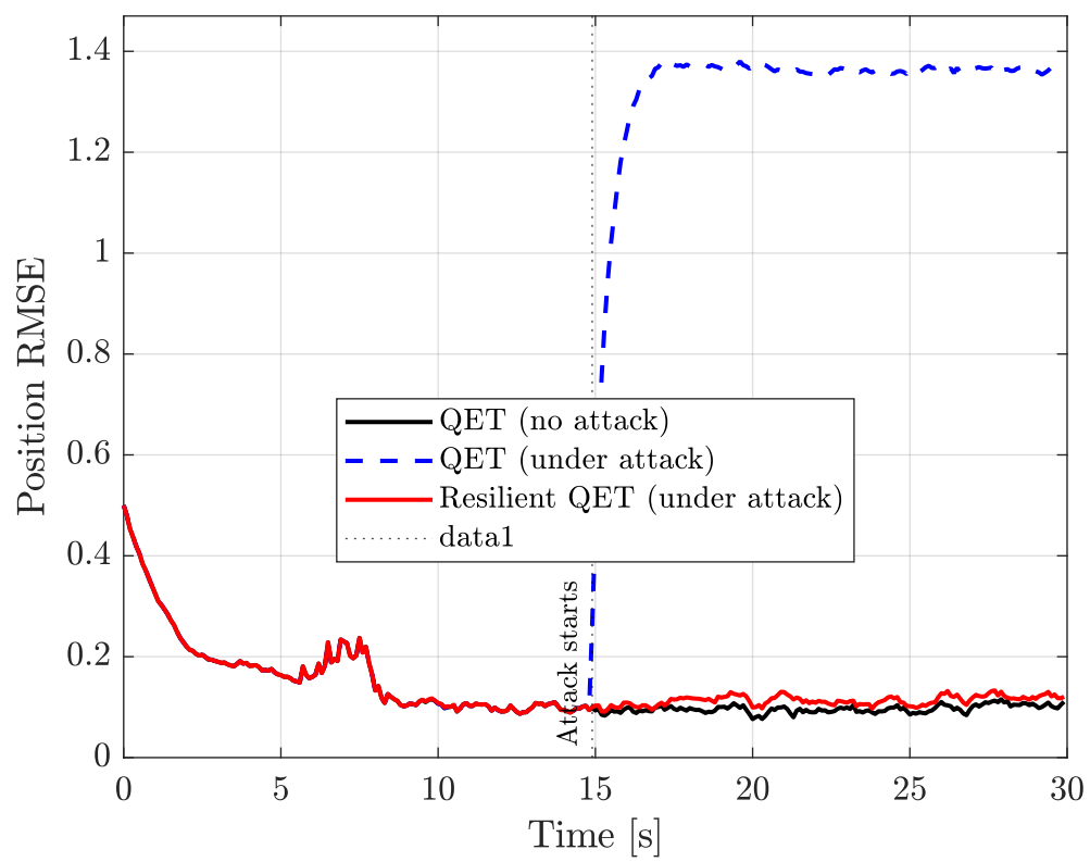
Estimation Performance under Sensor Attack
