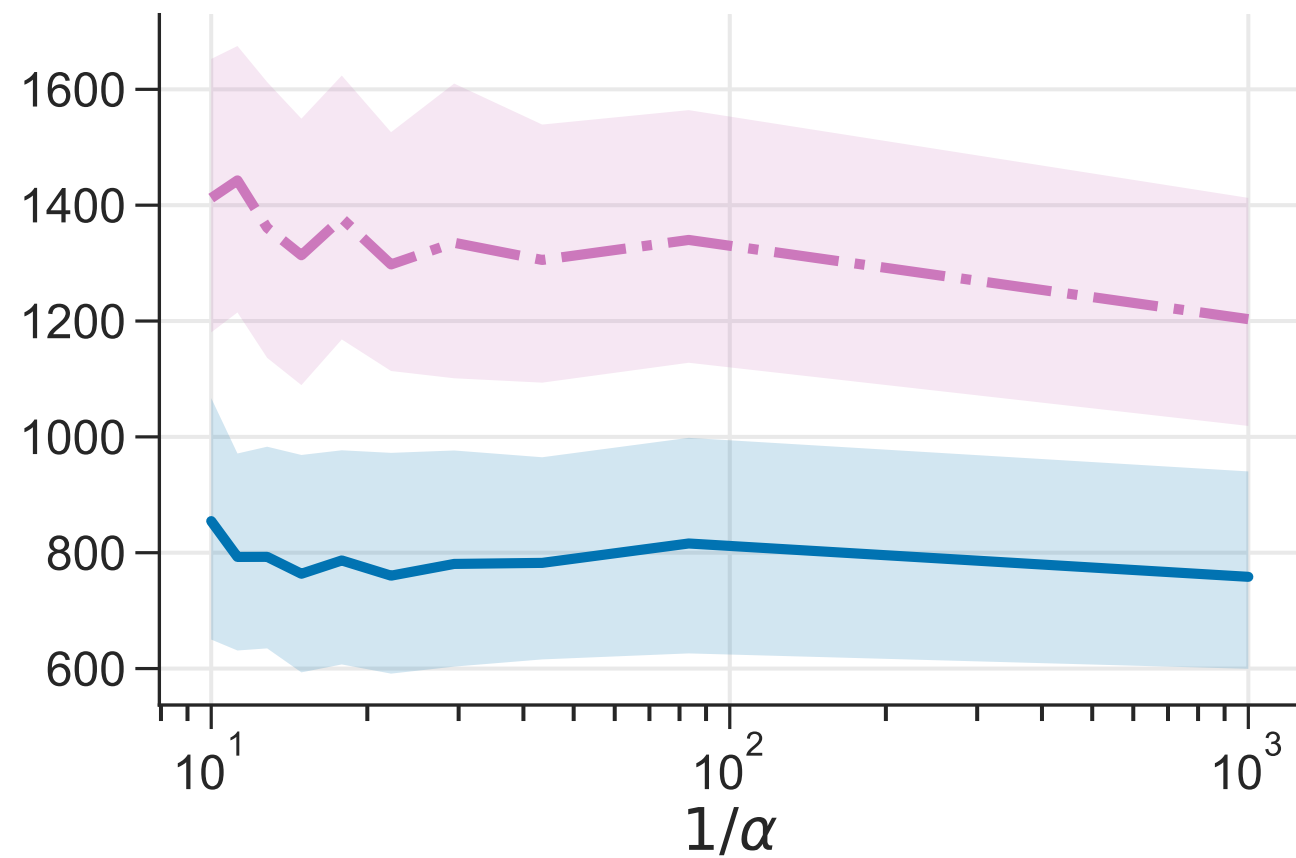
(a) Ridge MSE
