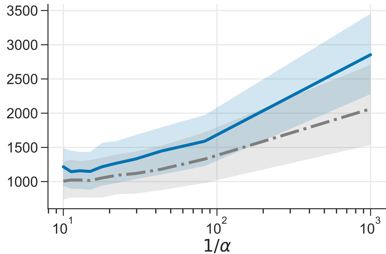
(b) Hard-thresholded ridge MSE
