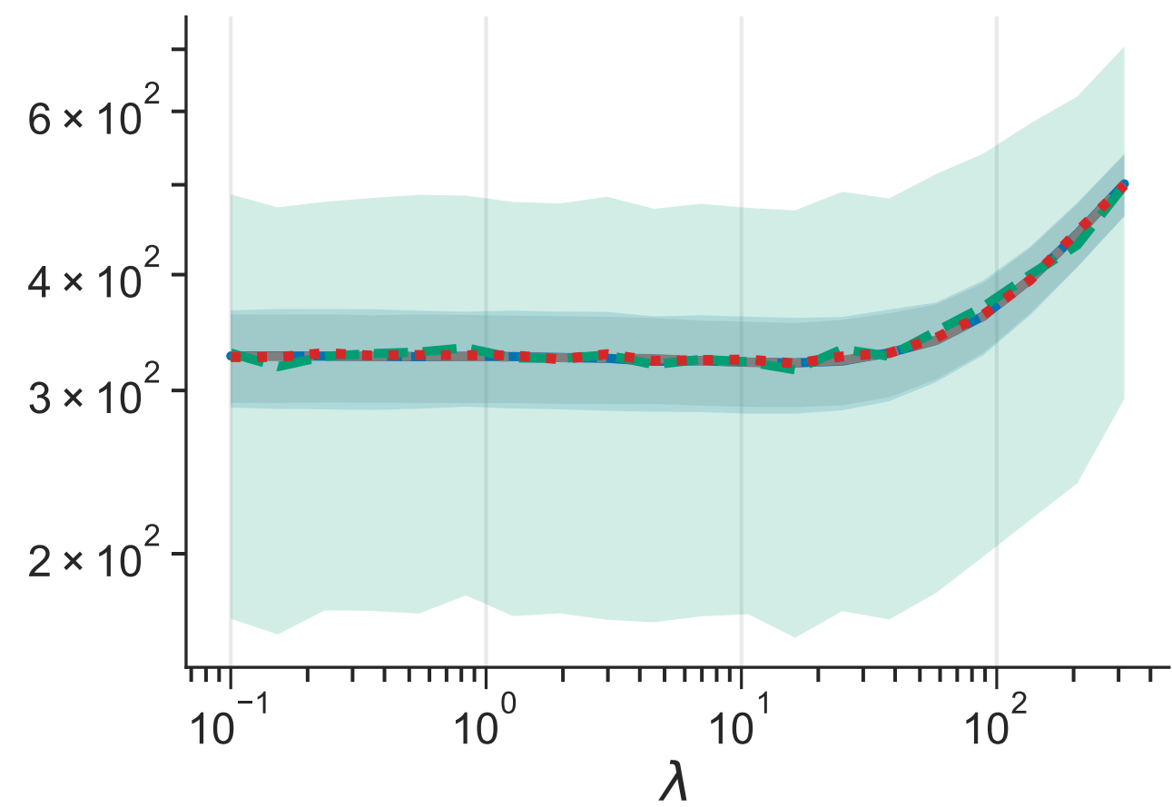
(c) Hard-thresholded ridge estimated risk versus \lambda
