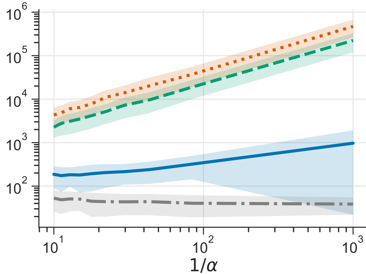
(b) Hard-thresholded ridge reducible variance
